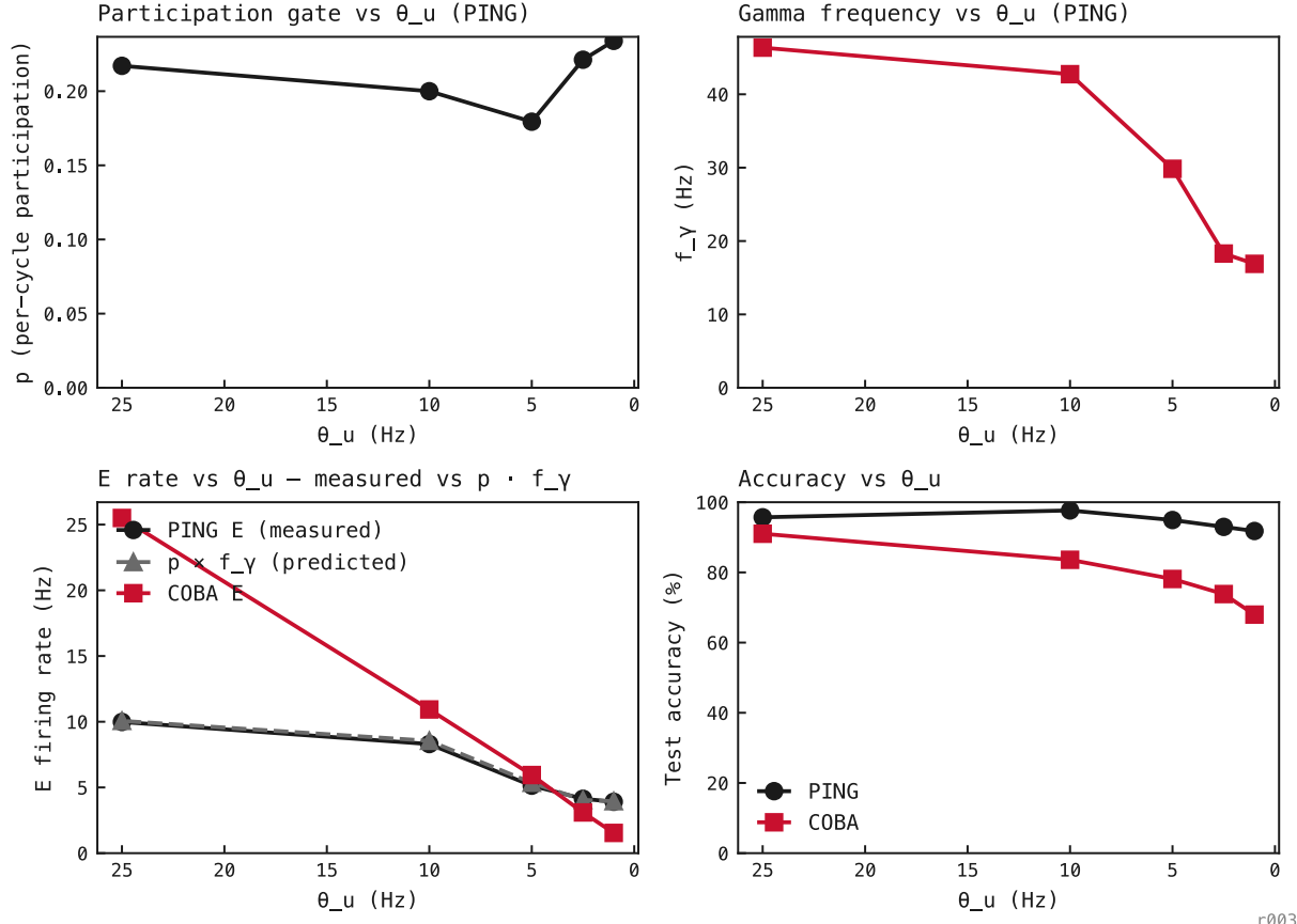
Figure 2: Five representative seed-42 (PING, \theta_u ) sweep checkpoints, 256 test trials each. p stays in 0.18–0.23 across the entire sweep (the architecture protects the participation gate), while f_\gamma slides from \approx 46 Hz to \approx 17 Hz as the penalty tightens. The grey dashed p \cdot f_\gamma curve overlays the measured E rate within 4%; the rate change is entirely in f_\gamma . PING accuracy holds at 92–98% the whole way; COBA’s collapses from 91% to 68%.
