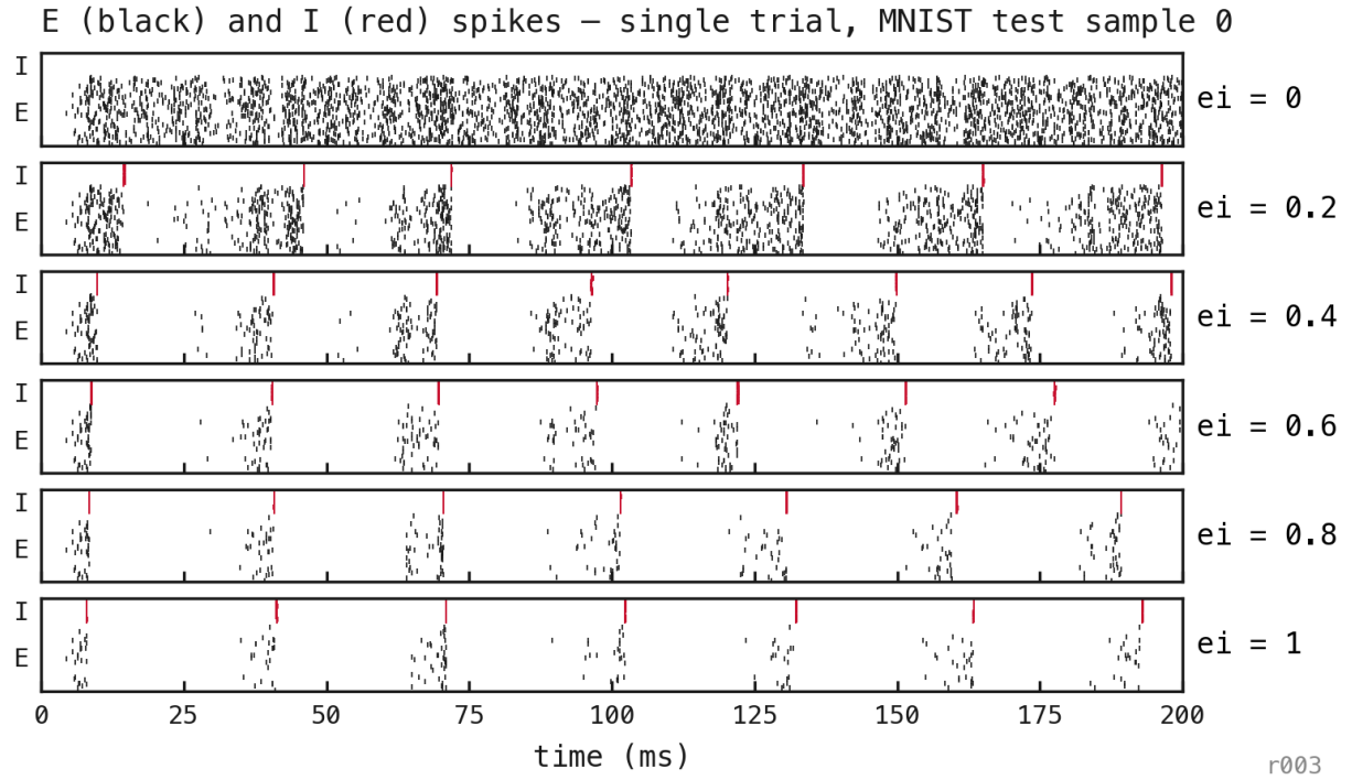
Figure 110: The full transition: trained COBA replayed at six inference-time ei\_strength values (same trial, same feedforward weights, a fresh I-loop each row). At ei = 0 the asynchronous-dense COBA pattern persists; by ei \approx 0.4 the same weights produce gamma cycles, sharpening toward ei = 1 . The rhythm appears continuously as the loop is wired in — no retraining at any point.
