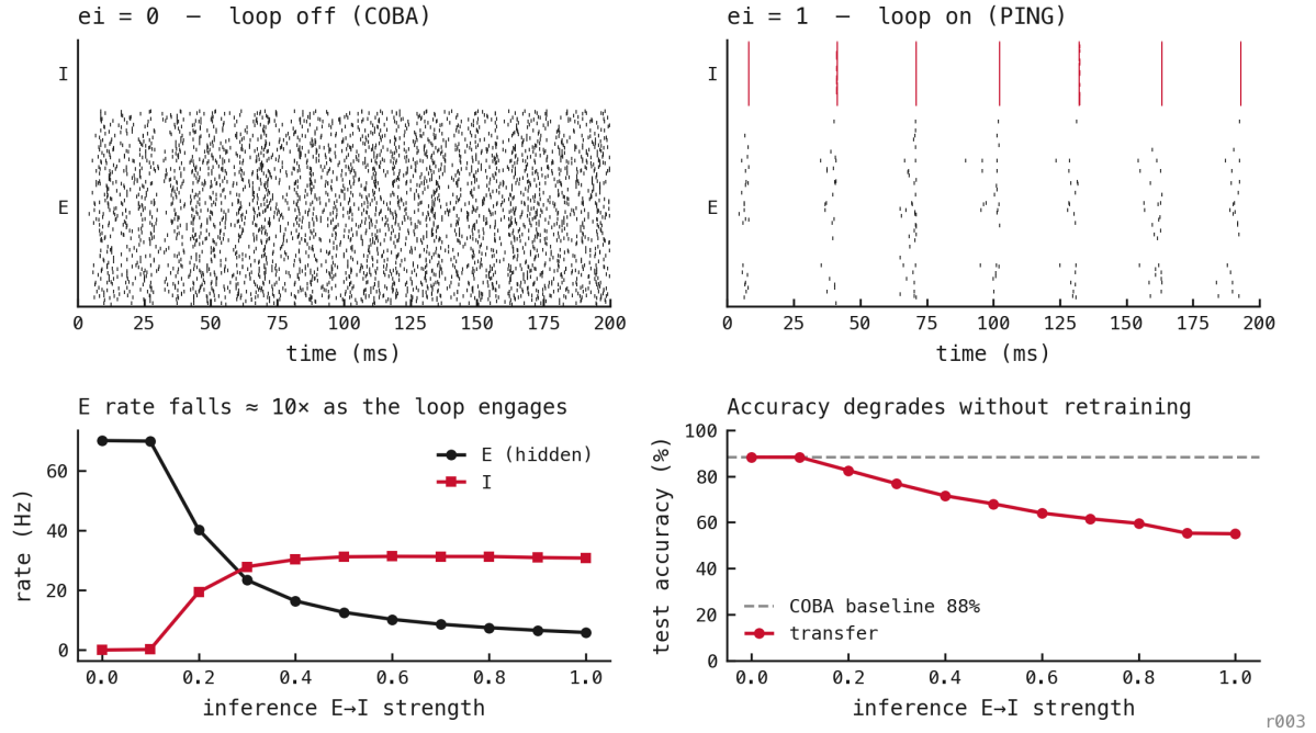
Figure 109: Switching the recurrent I-loop on at inference on a trained COBA network — no retraining, W^{EI}/W^{IE} freshly wired (the COBA checkpoint stores them at zero). Top — the same feedforward weights fire densely and asynchronously at ei = 0 (COBA) and in gamma bands at ei = 1 (PING); the gamma dynamics come from the inhibitory architecture, not from training. Bottom left — E rate falls \approx 10\times ( \approx 60 \rightarrow 5 Hz) as the loop engages while I rises to \approx 28 Hz; the suppression is continuous in loop strength. Bottom right — accuracy degrades without retraining, from the \approx 87\% COBA baseline to \approx 63\% at full strength (a \approx 24 pp cost). So the architecture supplies the rate-gating for free, but using it well needs training with the loop (nb025): the sparsity is architectural, the accuracy is learned.
