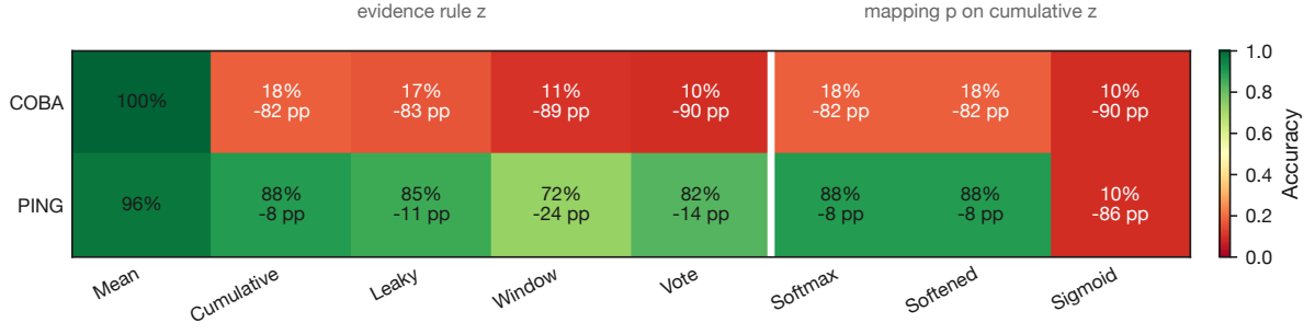
Figure 10: Decoder transfer screen. Each cell gives accuracy and, below it, the change from that network’s native mean-voltage decoder. The divider separates temporal evidence choices from mappings of the shared cumulative-count evidence.
