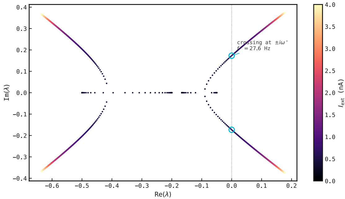
Figure 55: How to read it. Each dot is one eigenvalue \lambda of the Jacobian (28). Its horizontal position is the growth rate \text{Re } \lambda (negative means that mode decays, positive means it grows), and the dotted line at \text{Re } \lambda = 0 is the stability boundary: everything to its left is damped. Its vertical position is the oscillation frequency \text{Im } \lambda (zero = a non-oscillating mode, on the real axis). The Jacobian is 4 \times 4 , so each drive contributes four dots; sweeping I_{\text{ext}} (colour, dark→bright) drags them along the curves shown. Follow the upper and lower arms: one complex-conjugate pair lifts off the real axis and marches rightward, touching the boundary at \pm i\omega^* (cyan circles) when I_{\text{ext}}^* = 0.6 nA. That crossing is the Hopf, where the network tips from damping to amplifying, and the height of the crossing sets the rhythm, f^* = \omega^*/2\pi \approx 27.6 Hz. The other two eigenvalues stay left of the line throughout, so a single oscillation goes unstable: a simple Hopf. (A second pair reaches the axis only at far higher drive, above the recruitment cliff.)
