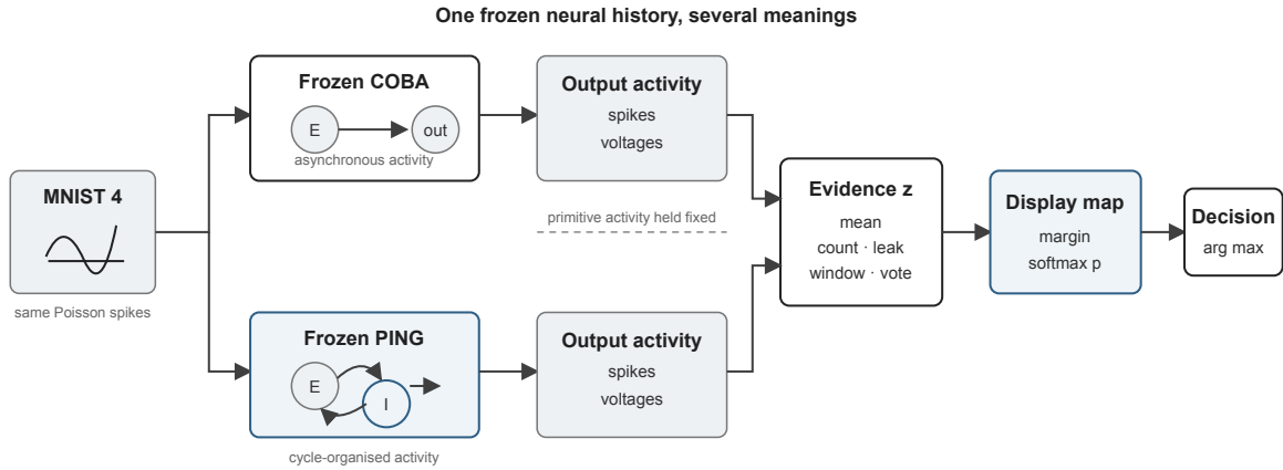
Figure 132: Shared decoder decomposition. Frozen activity enters a temporal evidence rule z , then an optional display mapping p , before the final argmax decision.
