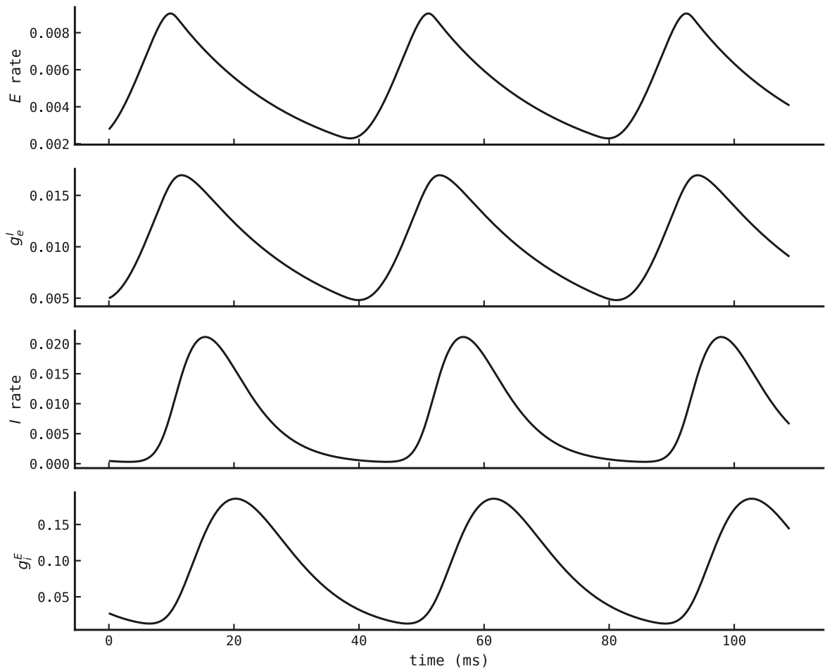
Figure 59: The four state variables over the limit cycle ( I_{\text{ext}} = I^* + 0.4 nA), in loop order E \rightarrow g_e^I \rightarrow I \rightarrow g_i^E . Each peaks after the one above it: g_e^I tracks the E rate almost rigidly (the near-degenerate pair of step 2), then drives I , which fills g_i^E , which shunts E : one round trip of the ring per gamma cycle.
