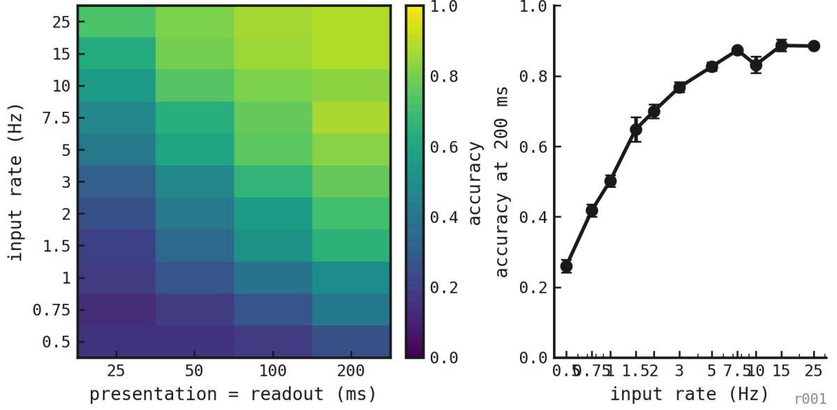
Figure 3: Held-out accuracy across matched presentation/readout durations and trained input rates. The right panel fixes duration at 200 ms to separate rate tolerance from integration time.
