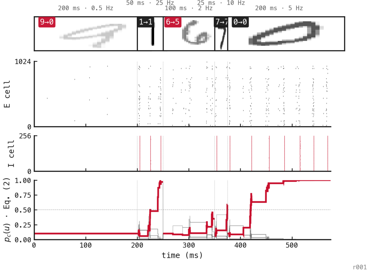
Figure 2: A five-digit stream classified by the native output-LIF spike-count readout. Counts reset at each boundary; hidden PING state continues. Thumbnail opacity increases with input rate, and badges show the true and predicted labels.
