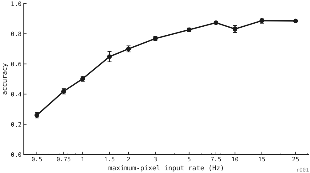
Figure 4: Input-rate psychometric with presentation and spike-count window fixed at 200 ms. Each rate contains 200 held-out digit presentations for each of three trained seeds.
