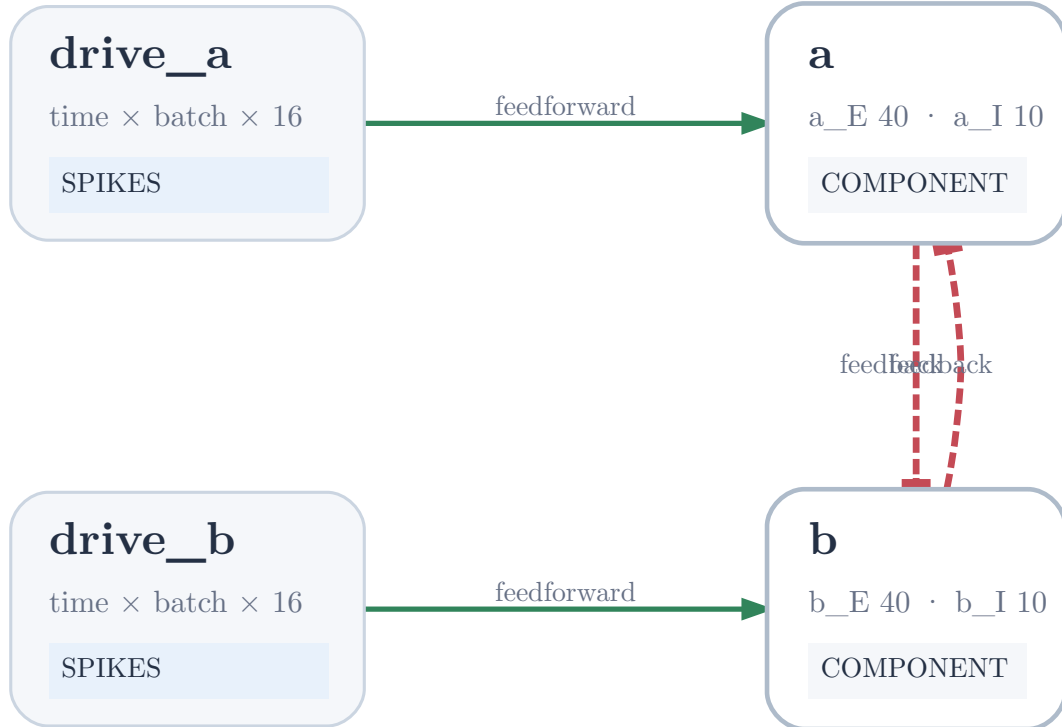
Figure 2: Representative reciprocal graph. Each inhibitory population sends a delayed GABA projection to the other circuit’s excitatory population; the two input nodes are independent.
