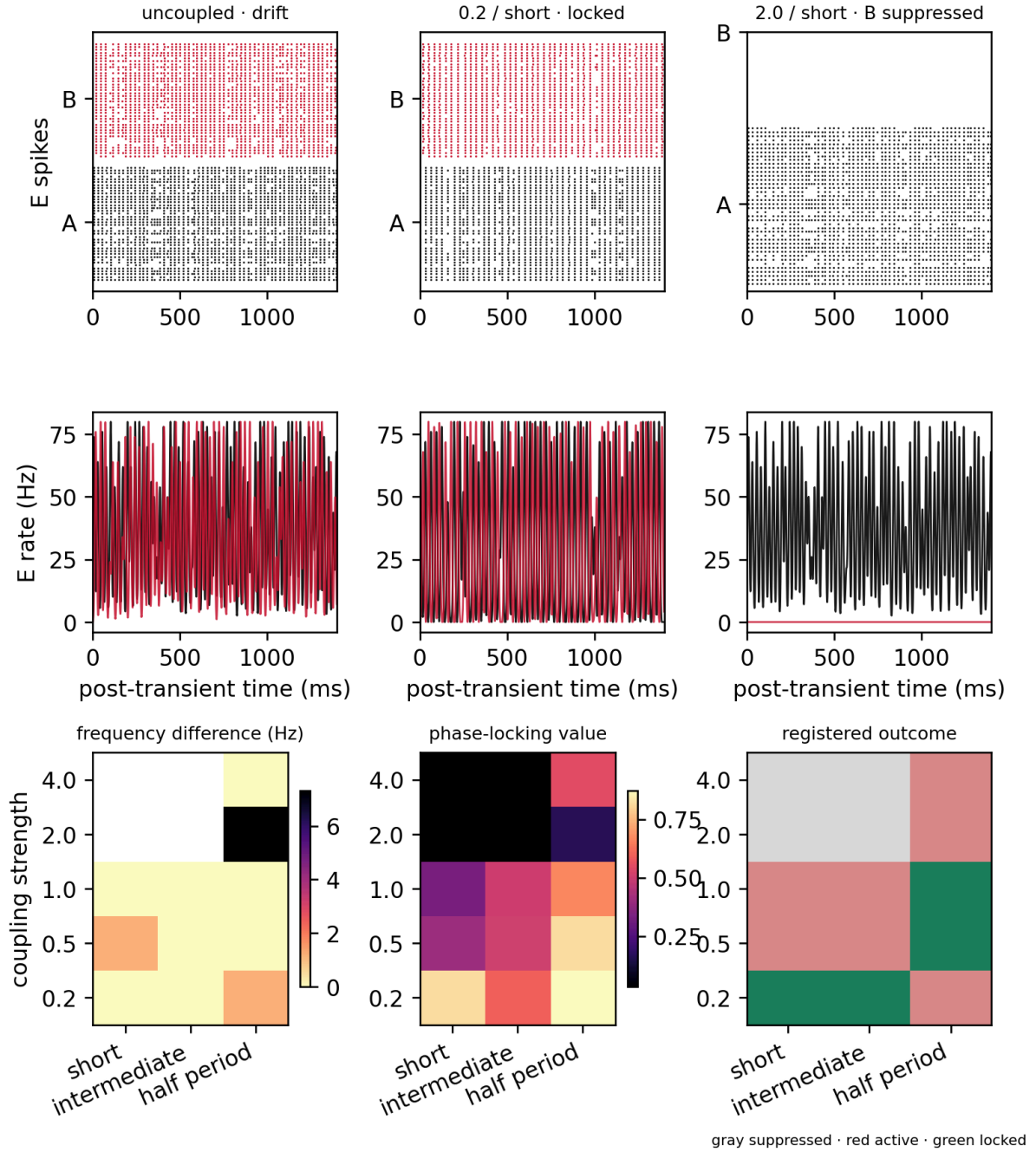
Figure 1: The mechanism in one view. Matched rasters and rates show uncoupled drift, active locking at strength 0.2 with short delay, and one-sided suppression at strength 2 with short delay. The maps below show the loss of frequency difference, rise in phase locking, contiguous registered locking region, and suppression boundary. Gray cells are suppressed, red cells remain active without passing every gate, and green cells are locked.
