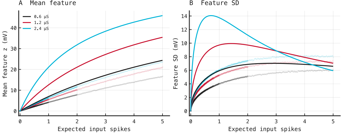
Figure 129: Analytical response moments over input drive. The horizontal axis matches Figure 2: expected input spikes are \lambda \frac{T}{1000} = rx \frac{T}{1000} . Panel A shows the analytical mean feature \mu_{\text{linear}(z)} from Equation 12a; Panel B shows the analytical SD \sqrt{\text{Var}_{\text{linear}(z)}} from Equation 18. Solid curves are analytical predictions; faint points are the corresponding empirical values from Figure 2. Black, red, and cyan denote probe conductances 0.6, 1.2, and 2.4 \mu\text{S} . The shared drive coordinate reveals mean overprediction directly and shows that the analytical and empirical SD maxima occur at different input drives.
