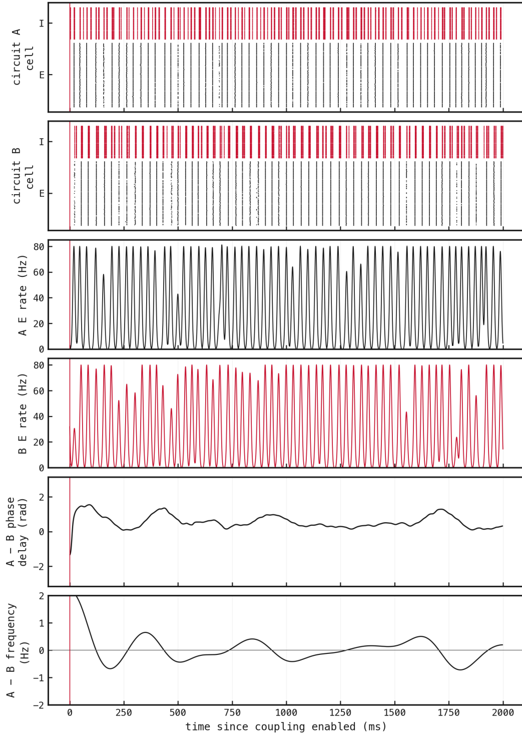
Figure 2: One continuous coupled trajectory from an already mature checkpoint. Reciprocal E \rightarrow I weight 0.22 and delay 10 ms are enabled at 0 ms; nothing else is reset. The first two panels show fixed samples of 100 E and 50 I neurons from circuits A and B. The next two show their full-population E rates on a common scale without overlap. The final two panels show 150 ms circularly smoothed A-minus-B phase delay and the corresponding instantaneous frequency difference, additionally smoothed over 75 ms. Phase wanders over the early and middle window while frequency difference changes sign. After 922.5 ms, phase remains bounded around a preferred lag and slow frequency difference remains centred near zero.
