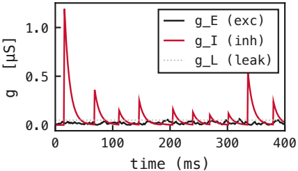
PING – recurrent loop active (ei-strength = 1.5) – E-neuron conductances (cell 73)
