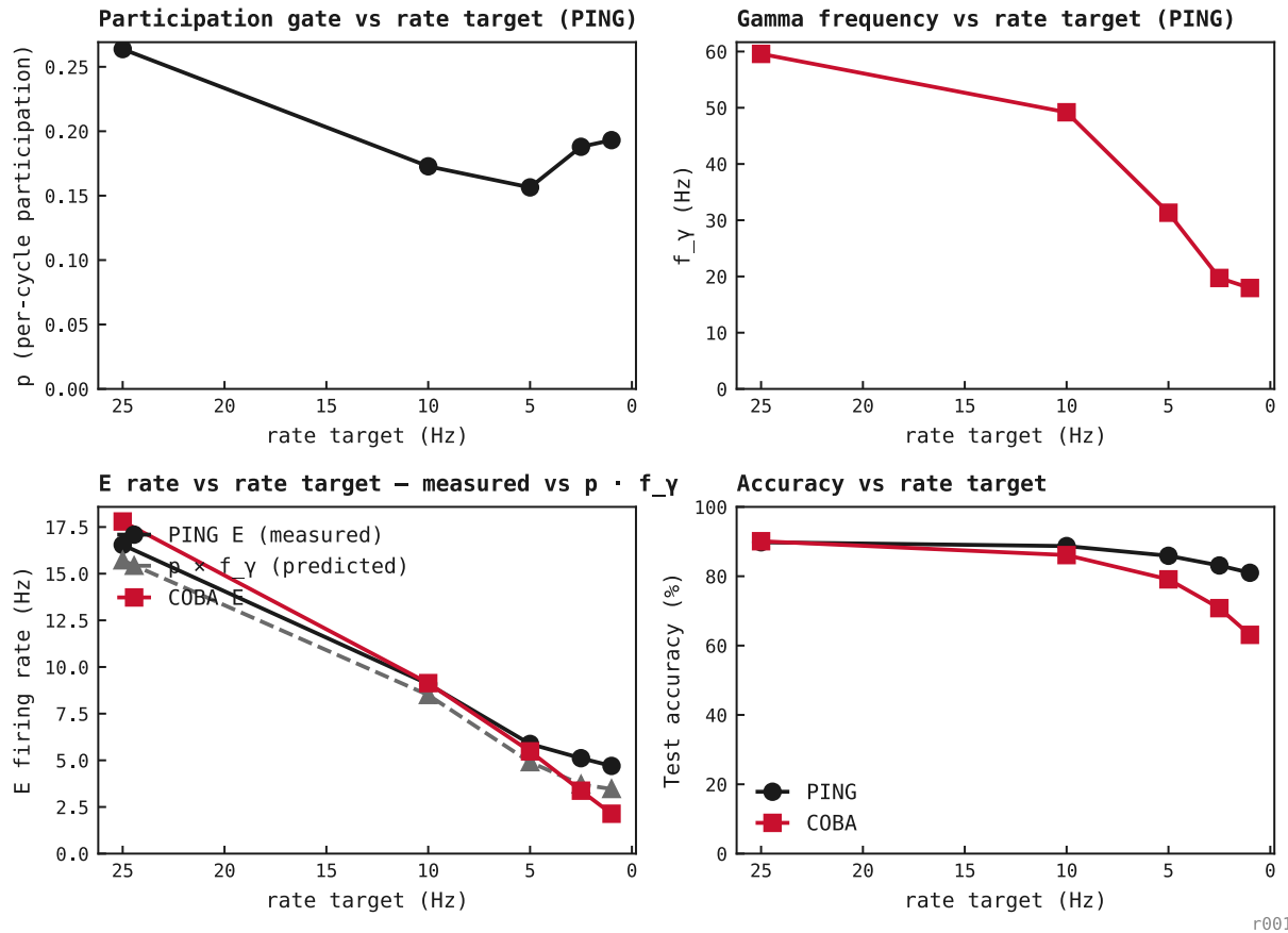
Figure 49: Five representative seed-42 PING rate-target checkpoints, 256 test trials each. p stays in 0.16–0.26 across the entire sweep (the architecture protects the participation gate), while f_\gamma slides from \approx 60 Hz to \approx 18 Hz as the penalty tightens. The grey dashed p \cdot f_\gamma curve overlays the measured E rate within 27%; the rate change is entirely in f_\gamma . PING accuracy holds at 81–90% the whole way; COBA’s collapses from 90% to 63%.
