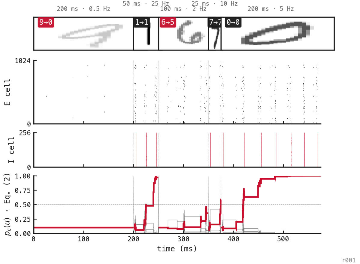
Figure 113: A five-digit stream classified by the native output-LIF spike-count readout. Counts reset at each boundary; hidden PING state continues. Thumbnail opacity increases with input rate, and badges show the true and predicted labels.
