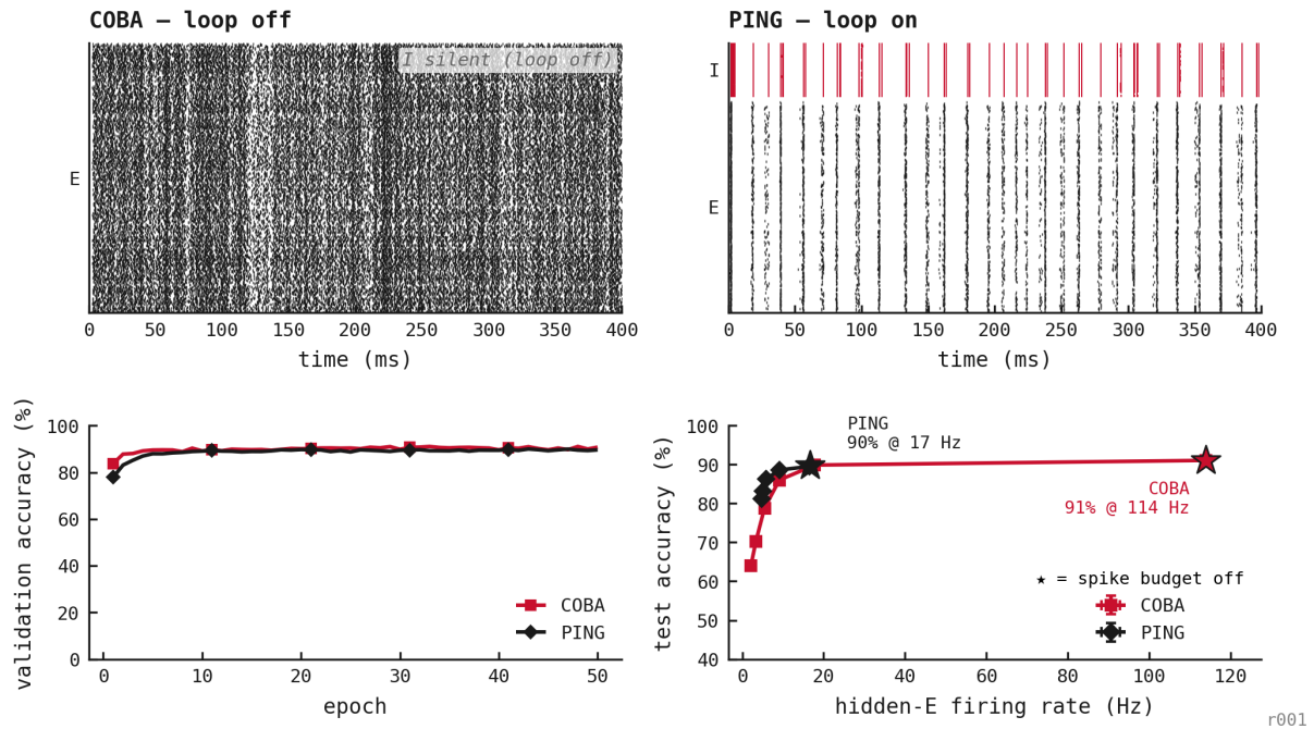
Figure 48: The headline comparison in one 2x2 frame (rasters, learning, and the accuracy-rate frontier together). Top: trained-baseline single-trial rasters on the same MNIST digit 0 input. COBA ( -ei-strength 0 ) fires densely and asynchronously at \approx 114 Hz (I silent, loop off); PING ( -ei-strength 1 ) fires in gamma bands at \approx 17 ms cadence ( \approx 17 Hz per E cell) with synchronous I bursts (red) above E (black), on the same architecture, parameter count, and recipe, with only PING’s recurrent E \leftrightarrow I matrices non-zero. Bottom left: validation accuracy per epoch (mean over three seeds); both reach \approx 90\% , so both learn the task. Bottom right: the accuracy-rate frontier across hidden-E rate ceilings (mean \pm SEM across three seeds at every point). PING sits up-and-left of COBA, the same accuracy at a fraction of the hidden-E rate, with the unpenalised operating points starred and labelled (PING 90% at \approx 17 Hz, COBA 91% at \approx 114 Hz). COBA red, PING black; E black and I red in the rasters. The headline of this entry: gamma gating buys an order-of-magnitude per-spike economy at matched accuracy.
