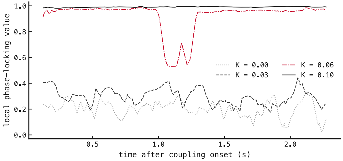
Figure 5: Synchrony over time after coupling onset at the four predeclared K values. Each trace is the median across 5 paired trials of the within-trial phase-locking value in a centered 250 ms window. Values near one indicate that relative phase remained nearly constant within that local window. This descriptive view exposes the trajectory directly without defining a binary synchronization boundary or requiring trials to settle at the same phase offset.
