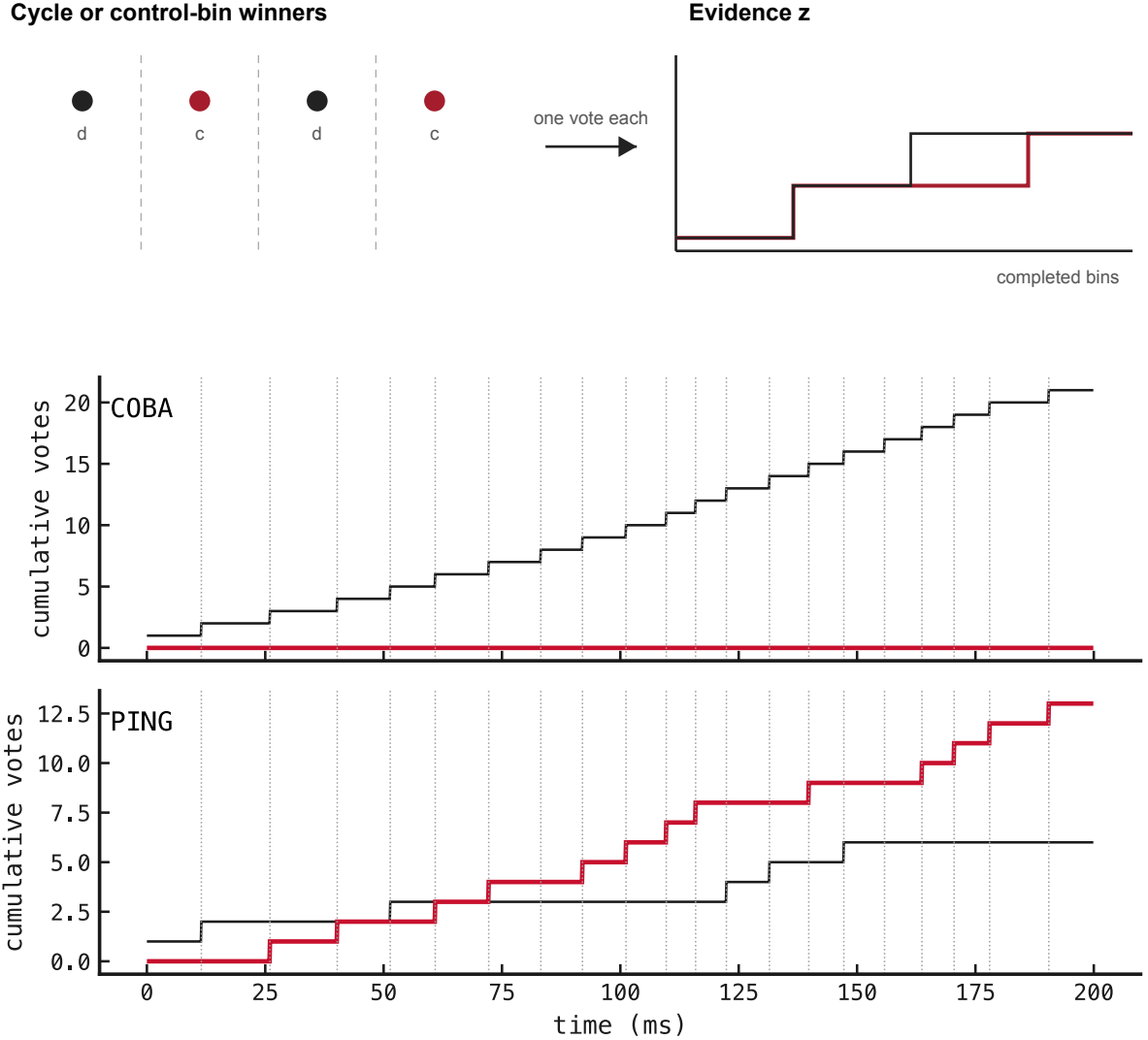
Figure 138: Cycle or matched-bin voting. Each interval names one winner before adding one vote. PING votes follow detected cycles and COBA votes use duration-matched controls.
