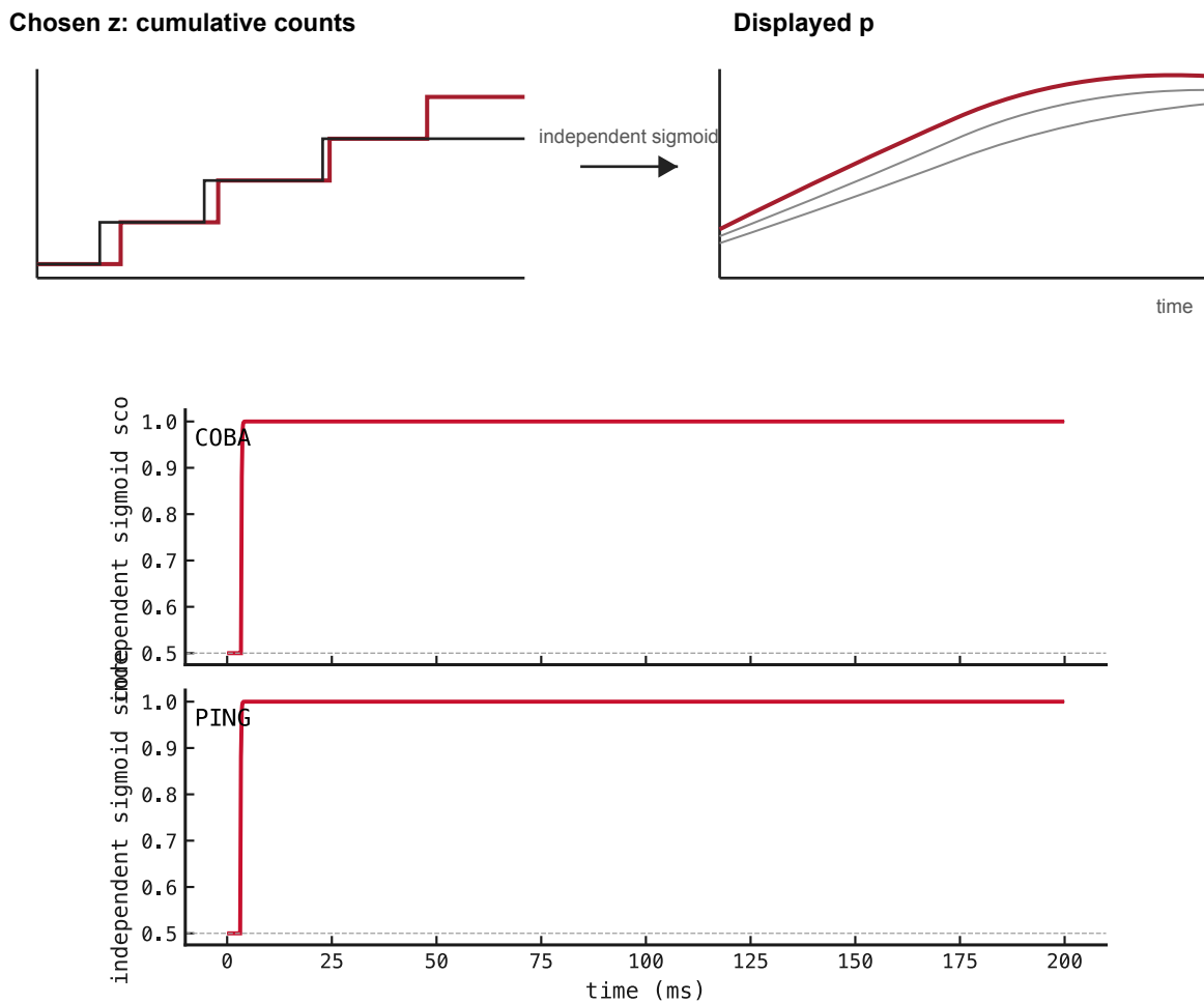
Figure 141: Independent sigmoid applied to cumulative spike counts. It retains the same z used by both softmax variants and reveals what is lost when classes no longer compete.
