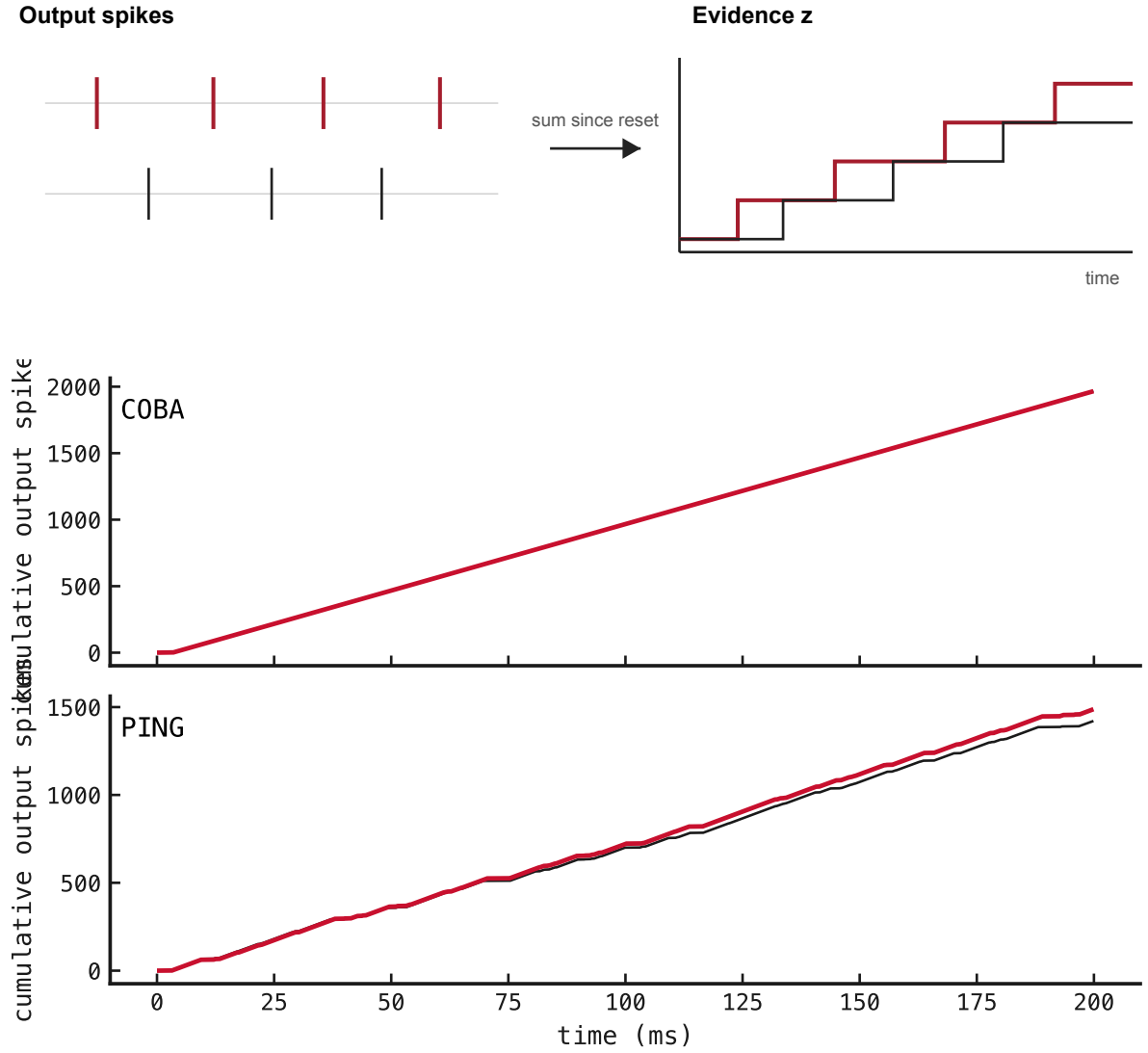
Figure 135: Cumulative-count decoder. Each output spike increments one class trace and no evidence decays; the staircase exposes early leads and later reversals.
