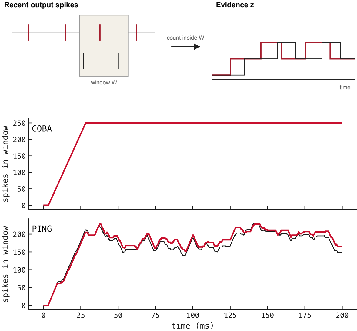
Figure 137: Sliding-window decoder. Evidence persists for 25 ms, then disappears abruptly when its spike leaves the window.
