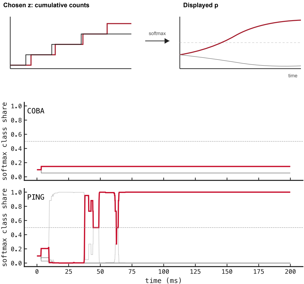
Figure 139: Ordinary softmax applied to cumulative spike counts. The measured mirror shows how an accumulating count margin becomes apparent confidence.
