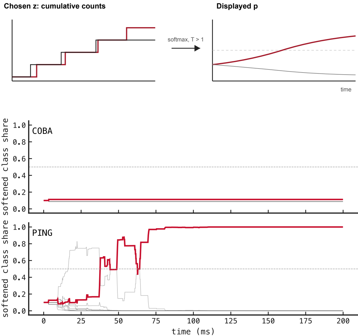
Figure 140: Temperature-softened softmax applied to the same counts. It differs from ordinary softmax only in temperature, isolating the effect of p .
