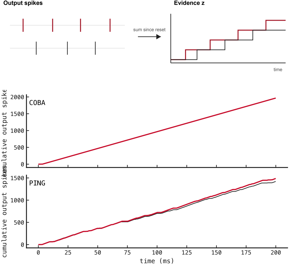
Figure 3: Cumulative-count decoder. Each output spike increments one class trace and no evidence decays; the staircase exposes early leads and later reversals.
