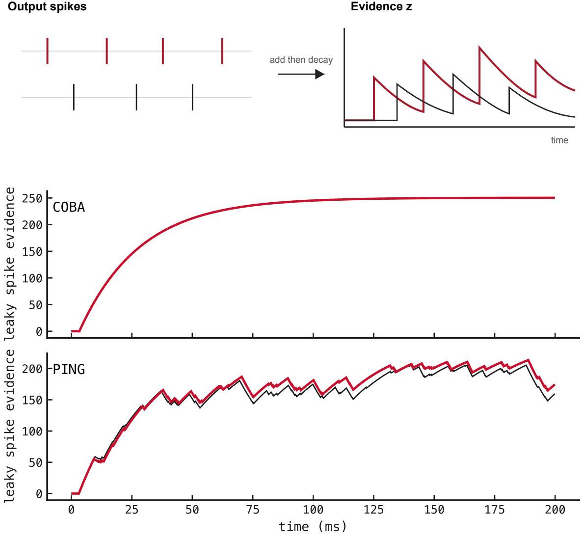
Figure 4: Leaky-count decoder. Spikes create upward steps and evidence decays smoothly between them, using the same leak factor for COBA and PING.
