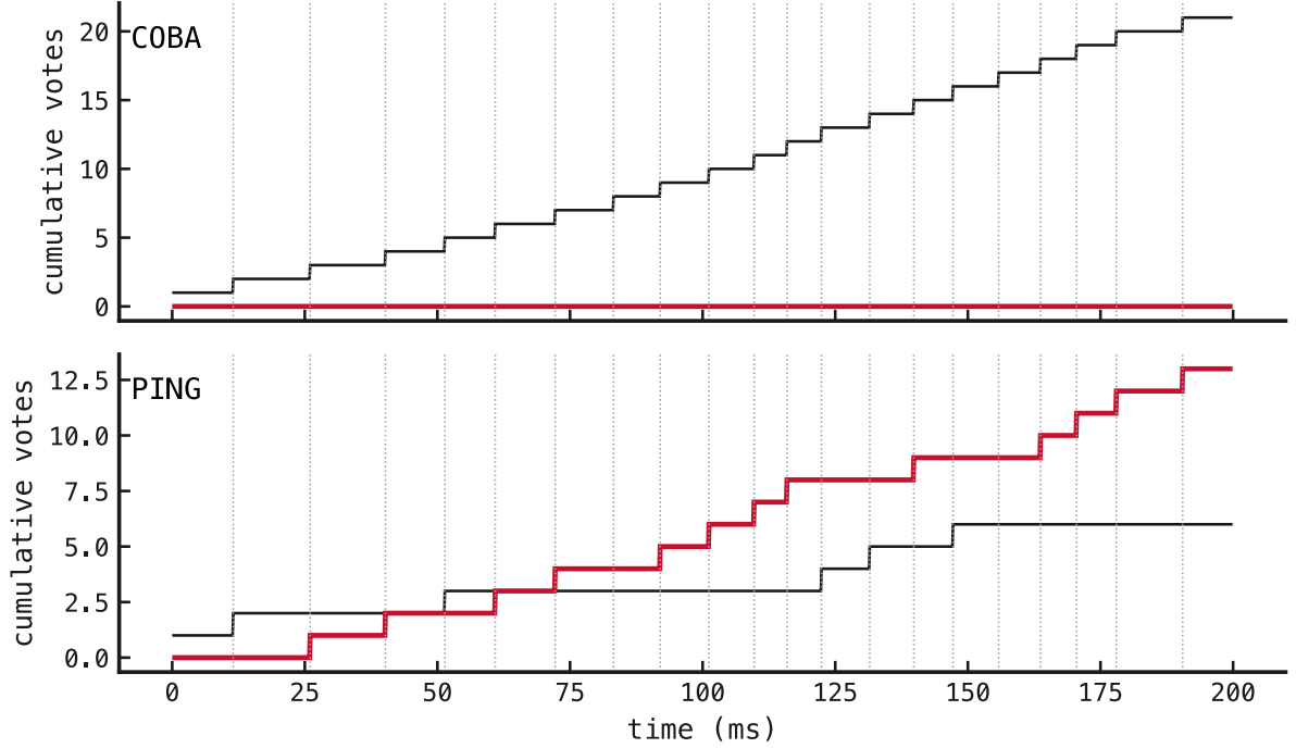
Figure 6: Cycle or matched-bin voting. Each interval names one winner before adding one vote. PING votes follow detected cycles and COBA votes use duration-matched controls.
