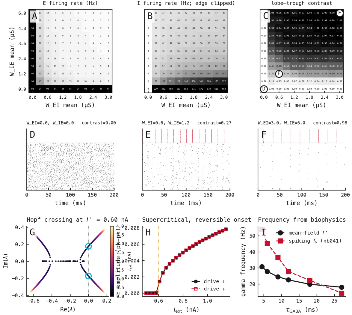
Figure 15: Gamma emerges through a smooth, reversible onset across the coupling plane, consistent with a supercritical Hopf bifurcation of the mean-field reduction. Nine panels (A–I). (A–C) Steady-state measurements across the 11 \times 11 W^{EI} \times W^{IE} coupling plane: mean excitatory firing rate (A), mean inhibitory firing rate (B), and the lobe-trough rhythmicity contrast R (C, §5.5), which is \approx 0 along the two COBA edges and rises to \approx 0.98 toward strong coupling. (D–F) Single-trial E (black) and I (red) rasters at three points sampled along the W^{IE} = 2W^{EI} diagonal (circled in C): the loop-disabled origin (D, asynchronous), weak coupling ( R < 0.5 , E), and strong coupling (F, sharp gamma volleys). (G–I) The four-dimensional conductance mean-field reduction (§5.3): a complex-conjugate eigenvalue pair crosses into the right half-plane at external drive I^* = 0.60 nA (G), locating a Hopf bifurcation at f^* \approx 27.8 Hz; the steady-state oscillation amplitude grows continuously across the onset with coincident up- and down-ramp branches (H), the signature of a supercritical, reversible transition; and the predicted gamma frequency falls with \tau_{\text{GABA}} in qualitative agreement with the spiking measurement (I). Source: exp054 (coupling-plane maps and mean-field, incorporating exp033); spiking f_\gamma from exp041.
