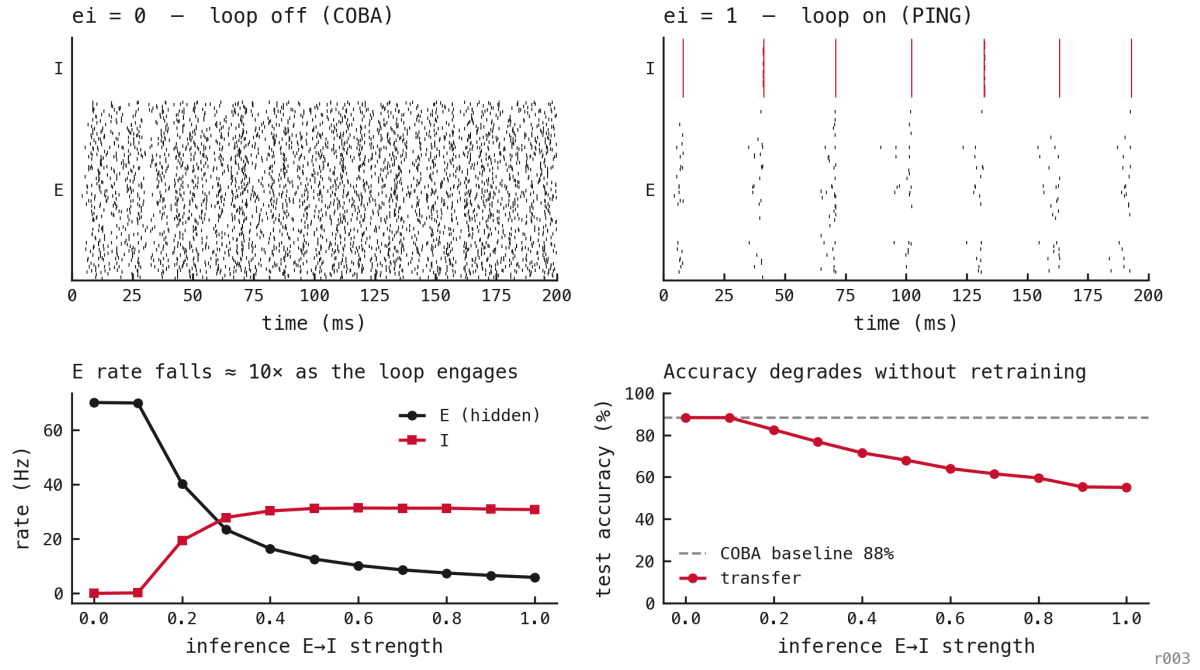
Figure 17: Engaging the recurrent loop at inference on a trained COBA network reproduces the PING firing-rate reduction with no weight update. A network trained in the COBA configuration is evaluated with the recurrent E \rightarrow I coupling scaled from ei = 0 (loop off, as trained) to ei = 1 (canonical loop strength), without retraining. Top: single-trial rasters at ei = 0 (dense, asynchronous, inhibitory population silent) and ei = 1 (gamma bands, synchronous inhibitory bursts). Bottom left: mean excitatory (black) and inhibitory (red) firing rates versus inference coupling strength; the excitatory rate falls approximately tenfold (from \approx 60 to \approx 5 Hz) as the inhibitory rate rises to \approx 28 Hz. Bottom right: test accuracy versus coupling strength, falling from the \approx 87\% COBA baseline to \approx 63\% at ei = 1 (a \approx 24 pp cost). The rate gating appears the instant the loop is wired in, whereas the accuracy loss reflects the absence of a feedforward compensation that only training in the presence of the loop provides.
