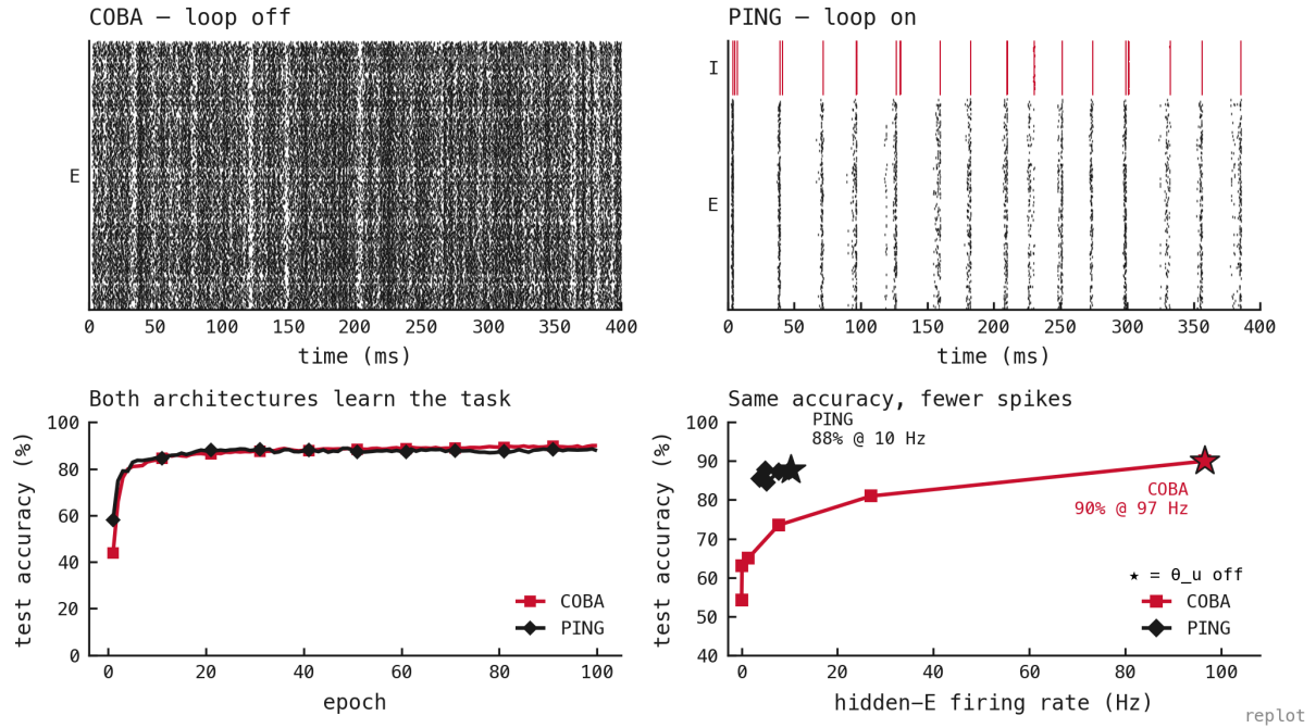
Figure 16: Trained PING matches COBA classification accuracy while operating at an order-of-magnitude lower excitatory firing rate. Both configurations were trained on MNIST by surrogate-gradient descent (§5.4). Top: representative single-trial rasters of the trained networks — COBA fires densely and asynchronously with the inhibitory population silent, whereas PING fires in gamma bands with synchronous inhibitory bursts (red) above excitatory spikes (black). Bottom left: test accuracy per epoch, both configurations converging to \approx 83\% . Bottom right: accuracy–rate frontier traced by sweeping the per-neuron spike-budget penalty \theta_u (§5.4); each marker is a trained network, plotting mean hidden-E firing rate (abscissa) against test accuracy (ordinate). PING lies above and to the left of COBA across the sweep. At the operating point with \theta_u disabled (starred), PING reaches \approx 83\% at \approx 3.8 Hz, against COBA’s \approx 90\% at \approx 56 Hz. Source: exp025 rate-attractor analysis in exp024.
