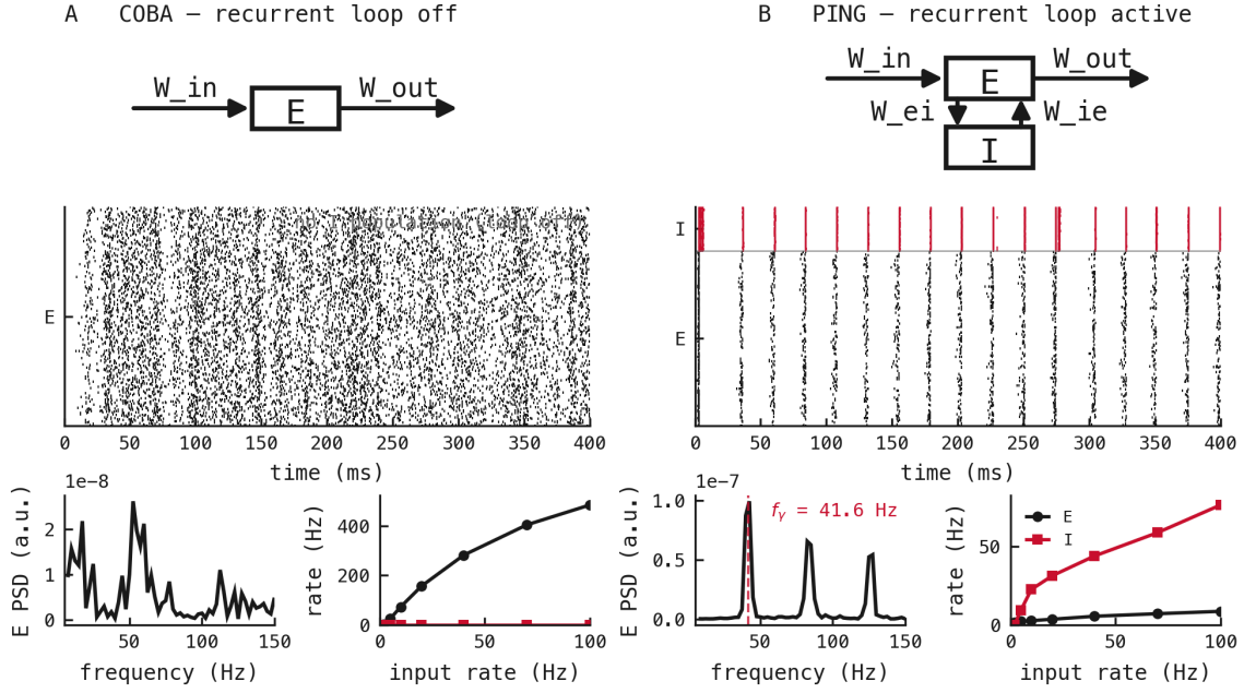
Figure 14: A single recurrent E \rightarrow I \rightarrow E loop simultaneously generates a gamma rhythm and clamps the excitatory firing rate. Free-running activity of the two-population conductance-based network (excitatory pool N_E = 1024 , inhibitory pool N_I = 256 ; canonical biophysical parameters, §5.1) under matched Poisson drive, in two configurations. (A) COBA baseline with the recurrent loop disabled ( W^{EI} = W^{IE} = 0 ): input projects to the excitatory (E) population only. The E spike raster is asynchronous, the Welch power spectral density (PSD) of the summed E population shows no gamma-band peak, and the excitatory f - I curve saturates near 270 Hz under strong drive. (B) PING configuration with the loop engaged ( E \rightarrow I via W^{EI} , I \rightarrow E via W^{IE} ; no I \rightarrow I or E \rightarrow E synapse): the inhibitory (I) population fires synchronous bursts, the E raster forms gamma bands, the PSD shows a discrete peak at f_\gamma \approx 25 Hz, and on axes shared with (A) the E rate is held approximately an order of magnitude lower across two decades of input drive while the I rate rises to \approx 64 Hz. Source: exp023.
