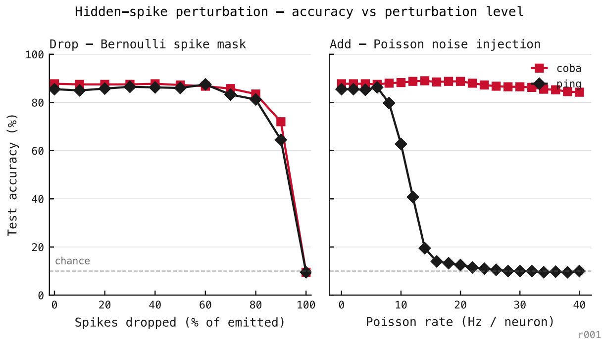
Figure 22: The gating is robust to spike deletion but fragile to spike addition — the expected signature of a phase-based code. A trained PING network is perturbed at inference (no retraining); accuracy is plotted against perturbation level. Left: deletion of a random fraction of emitted spikes. PING retains \approx 82\% accuracy — essentially its unperturbed value — through 80% deletion, degrading only as the network approaches silence. Right: addition of Poisson spikes, expressed as a fraction of each population’s baseline rate. PING accuracy falls sharply, reaching chance between \approx 15 and 65% added noise, because off-phase spikes drive the inhibitory pool at arbitrary phase and dissolve the rhythm. COBA (red), having no rhythm to protect, shows the mirror-image asymmetry: tolerant to addition, intolerant to deletion. Source: exp037.
