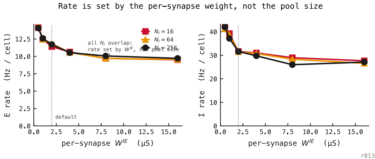
Figure 21: The firing-rate reduction is set by the strength of each inhibitory synapse, not by the size of the inhibitory pool. Per-cell firing rates as a function of the per-synapse I→E weight W^{IE} (0.5–16 \mu\text{S} ), swept independently at three inhibitory pool sizes N_I \in \{16, 64, 256\} . Left: excitatory rate, falling from \approx 14 Hz at W^{IE} = 0.5 \mu\text{S} to \approx 9.6 Hz at W^{IE} = 16 \mu\text{S} . Right: inhibitory rate, falling from \approx 42 to \approx 27 Hz. In both panels the three pool-size curves are superimposed, so the rate is governed by the per-synapse inhibitory gain rather than by interneuron count. The dashed vertical line marks the canonical W^{IE} = 2 \mu\text{S} . Source: exp047.
