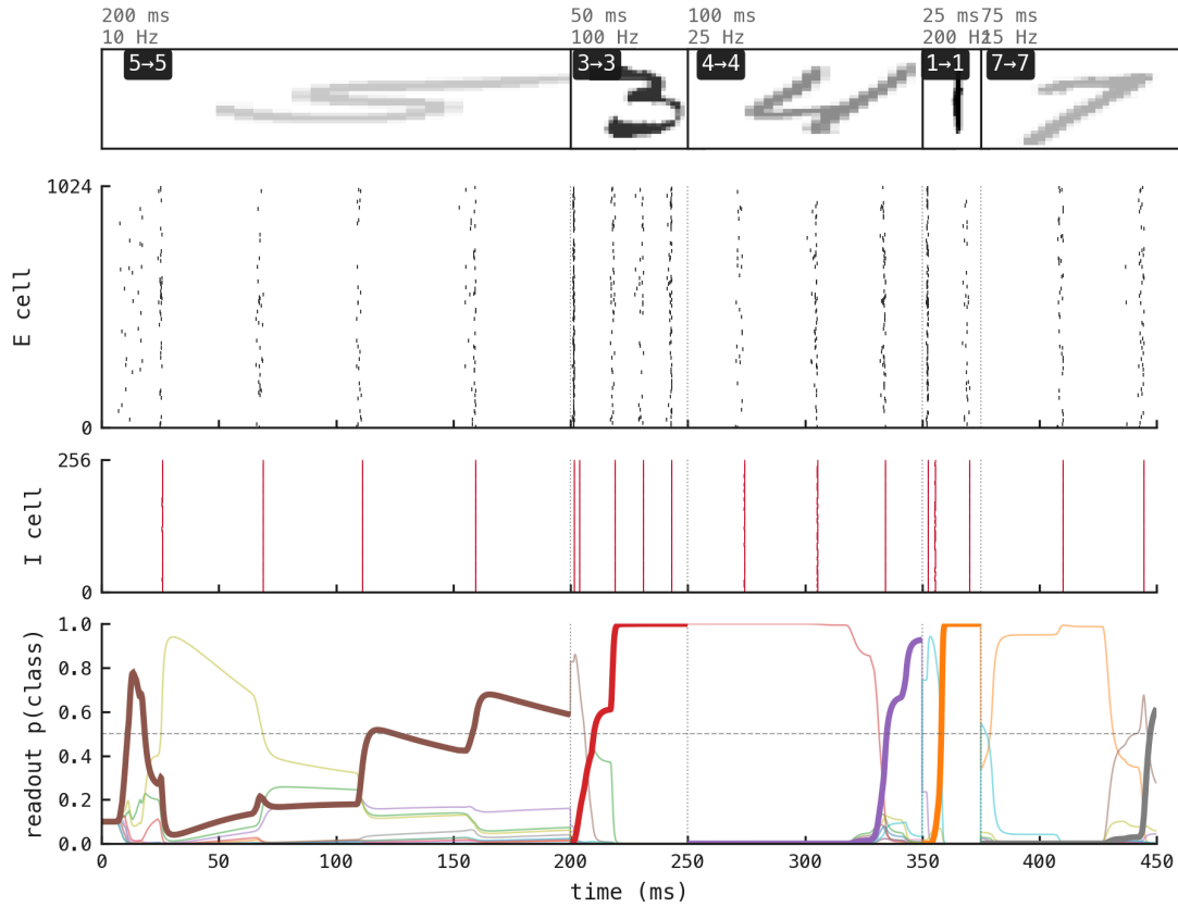
Figure 25: A PING network trained on isolated digits classifies a continuous, unsegmented stream whose presentation timing varies from segment to segment. A single input stream concatenates five MNIST digits, each with its own presentation duration (25–200 ms) and Poisson input rate (10–200 Hz); the network is given no segmentation cue and is not retrained. Top: the five digit thumbnails with their per-segment (duration, rate) and predicted labels; thumbnail opacity indicates input rate. Below: hidden excitatory and inhibitory rasters, showing gamma cycles maintained throughout — sparser under weak drive, denser under strong drive — and the sliding leaky-integrator readout traces, which identify each segment cleanly.
