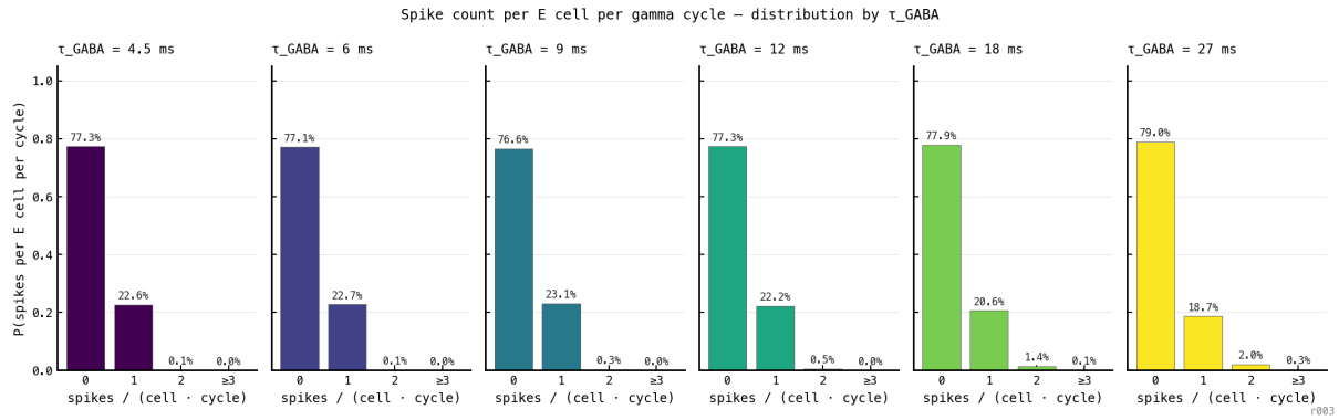
Figure 20: The affine rate law follows from a near-binary per-cycle firing statistic: each excitatory cell contributes at most one spike per gamma cycle. Excitatory spikes were resolved into (cell, cycle) pairs by assigning each spike to the gamma cycle inferred from peaks of the population inhibitory-burst rate (§5.5). Each panel shows the distribution of spikes per pair — 0, 1, 2, or \geq 3 — at one value of \tau_{\text{GABA}} . Across the sweep, P(0) \approx 77\% , P(1) \approx 22\% , and the multi-spike fraction ( \geq 2 ) stays below \approx 3\% ; pooled over all conditions, 99.45% of pairs contain at most one spike. Source: exp046.
