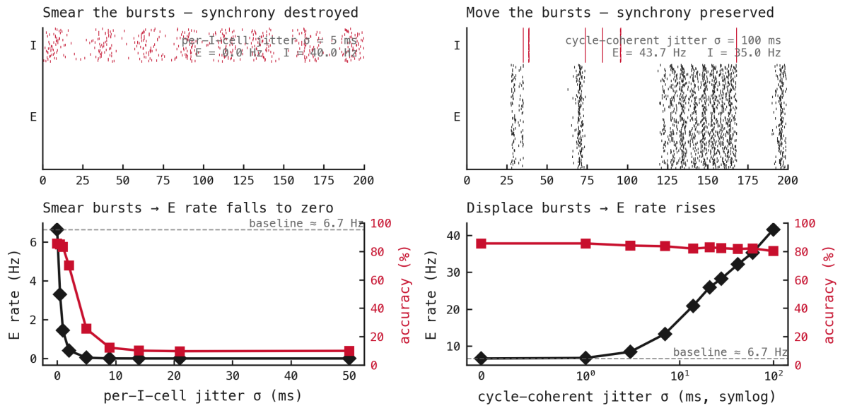
Figure 23: Two inhibitory-jitter manipulations that hold the mean inhibitory rate fixed drive the excitatory rate in opposite directions, isolating timing from level. The trained PING inhibitory spike train is perturbed at inference while the mean per-cell inhibitory rate is held constant. Top: single-trial rasters (E black, I red). Bottom: mean excitatory rate (black) and accuracy (red) versus jitter magnitude \sigma . Left: per-cell jitter ( \sigma = 5 ms) smears each burst into a continuous shunt; the excitatory rate falls to \approx 0 Hz (inhibitory rate \approx 40 Hz) and accuracy falls to chance. Right: cycle-coherent jitter ( \sigma = 100 ms) displaces whole bursts while preserving within-burst synchrony; the excitatory rate rises from \approx 8 toward \approx 50 Hz (inhibitory rate \approx 35 Hz) and accuracy holds near 80%. Identical mean inhibition, opposite excitatory outcome: the gate is the phase structure of inhibition, not its level. Source: exp042.
