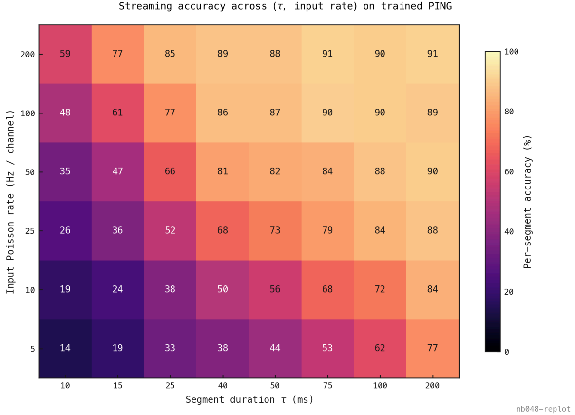
Figure 26: Classification requires an integration time of order one gamma cycle, identifying the cycle as the temporal quantum of the readout. Per-segment streaming accuracy across the grid of presentation duration \tau (abscissa) and input rate (ordinate), averaged over three seeds and 1,200 segments per grid cell. For \tau \leq 15 ms, accuracy does not exceed \approx 80\% at any input rate — a sub-cycle floor at \approx 0.4T_\gamma , with gamma period T_\gamma \approx 40 ms at f_\gamma \approx 25 Hz — and saturates by \tau \approx 40 – 50 ms ( \approx 1T_\gamma ). Above the floor, iso-accuracy contours run diagonally, so accuracy is approximately a function of the product \tau \cdot \text{rate} . The trained operating point ( \tau = 200 ms, 25 Hz) reaches 88%, interior to a broad high-accuracy plateau. Source: exp048.
