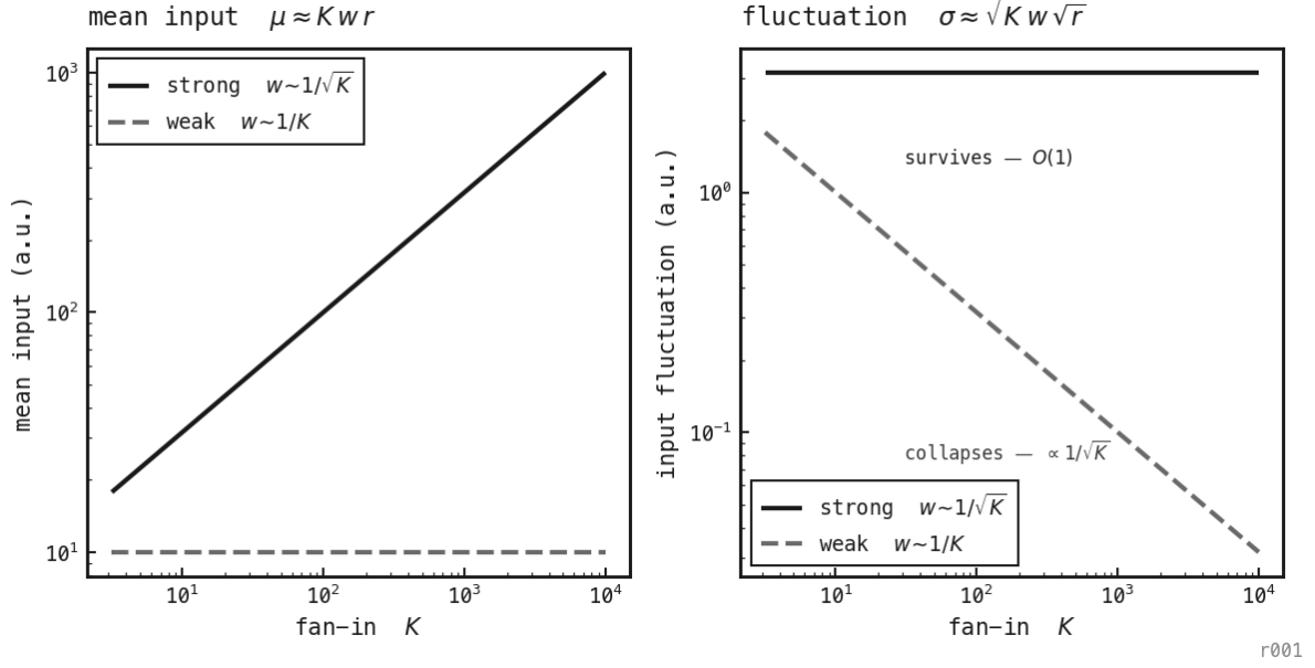
Figure 177: Equations (3)–(4) made visual. Left: the mean recurrent input \mu — under strong coupling it climbs \propto \sqrt{K} (so each population's drive is huge and must cancel); under weak coupling it is flat. Right: the fluctuation \sigma , and the punchline — under strong coupling it stays O(1) as the network grows (irregular firing survives), while under weak coupling it decays \propto 1/\sqrt{K} to zero (the network goes deterministic). Analytic; no simulation.
