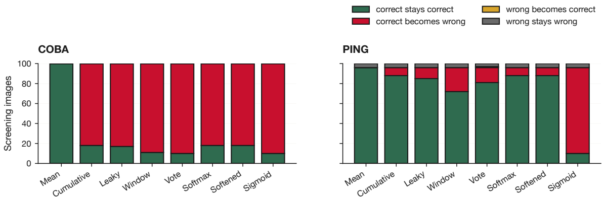
Figure 143: Decision transitions relative to native decoding. Green is preserved correctness; red is a native correct decision broken by the alternative. Yellow denotes a repair and grey a prediction that remains wrong.
