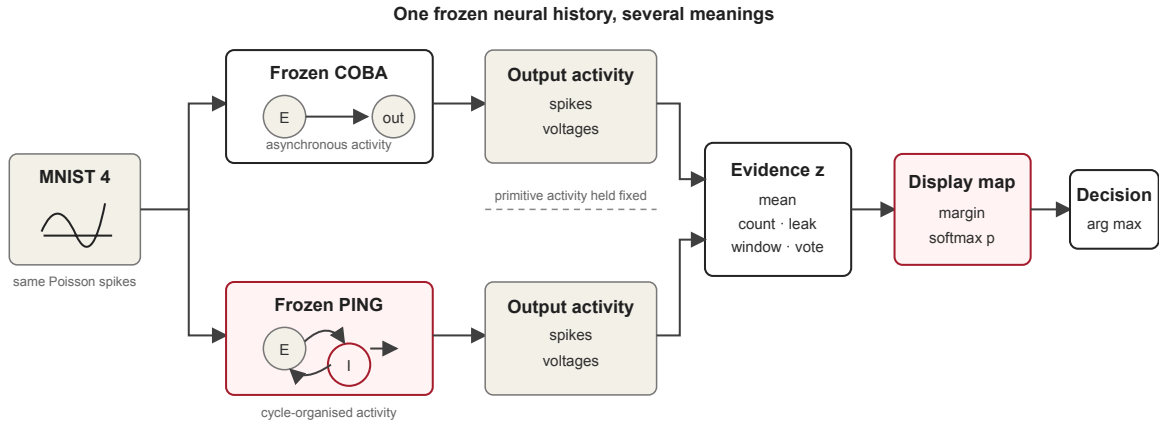
Figure 133: Decoder decomposition. Frozen COBA and PING networks produce output spikes and voltages. A temporal evidence function z compresses that activity, an output mapping p displays the resulting competition, and the decision selects the largest final score.
