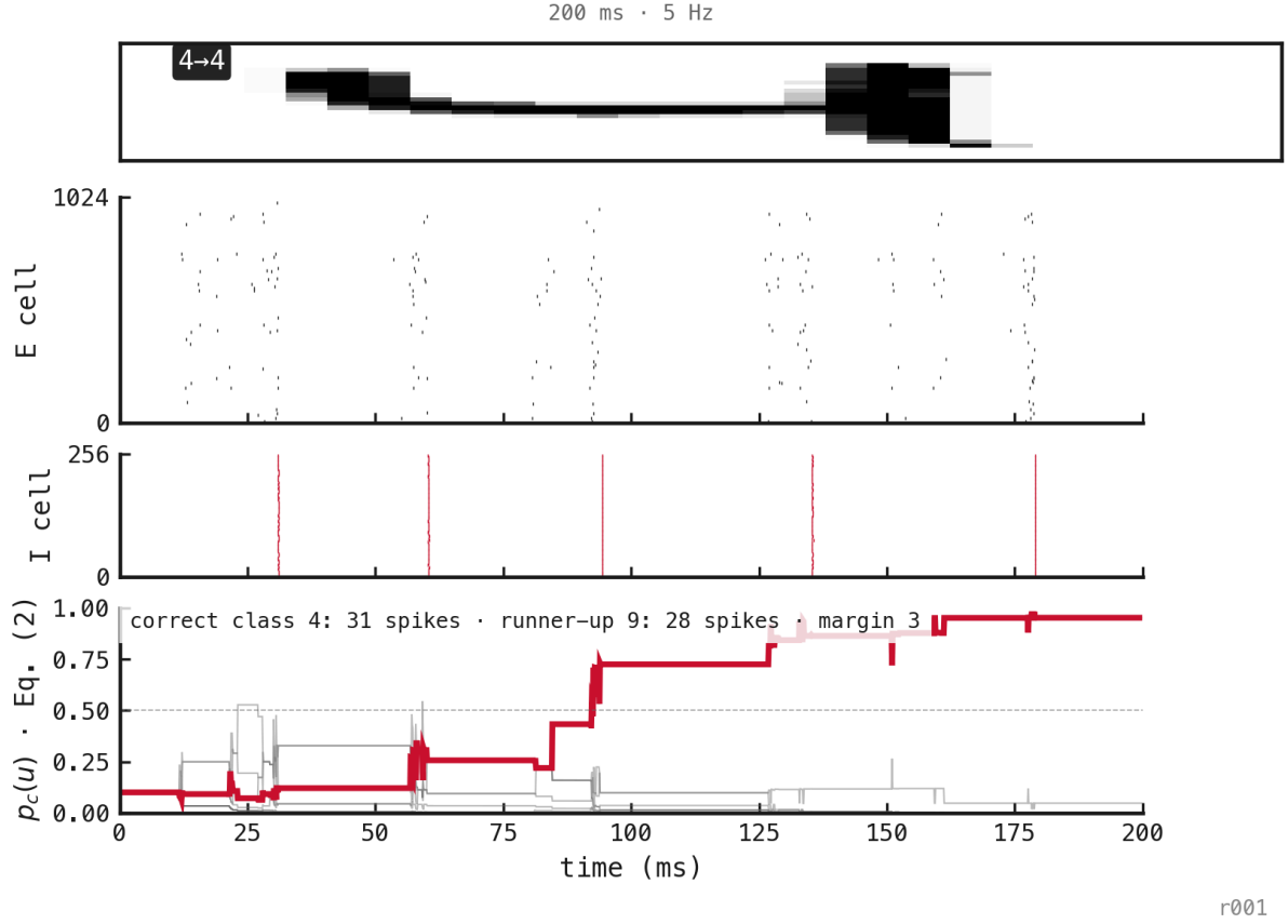
Figure 111: A correctly classified 200 ms presentation at a maximum-pixel input rate of 5 Hz, selected as the first success in the pre-existing matched stream. The output readout resets at the boundary while hidden PING state remains continuous. The top badge gives the true label and final prediction. The middle panels show E- and I-cell spike rasters. The lower panel shows p_{c(u)} from Equation 2; the true and winning class is red, and the annotation gives its final count, the runner-up count, and the winning margin. Equation 2 visualizes the cumulative integer counts z_{c(u)} from Equation 1 and is not a calibrated posterior probability. The plotted traces apply softmax to these cumulative counts. Softmax does not measure how much evidence exists in absolute terms; it shows how that evidence is distributed among the competing classes. Adding the same number of spikes to every class leaves the traces unchanged. What matters is the difference between their counts. For any two classes c and d ,
