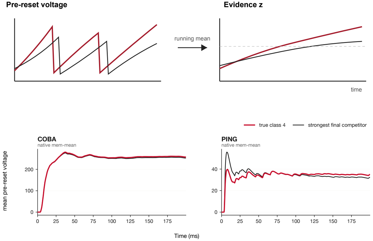
Figure 134: Mean-voltage decoder. The diagram shows pre-reset voltages entering a running temporal mean; the measured mirror shows the resulting frozen COBA and PING trajectories.
