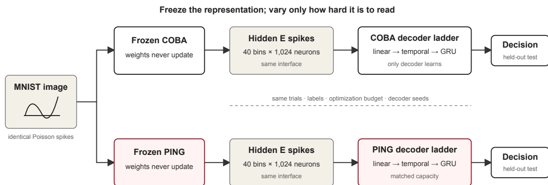
Figure 145: Experimental interface. Both networks receive the same input and expose the same 40 by 1,024 binned excitatory-spike representation. Only the separately fitted downstream decoder may learn.
