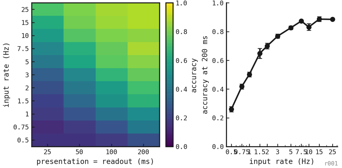
Figure 114: Accuracy across matched presentation/readout durations and input rates, with the 200 ms rate psychometric shown separately.
