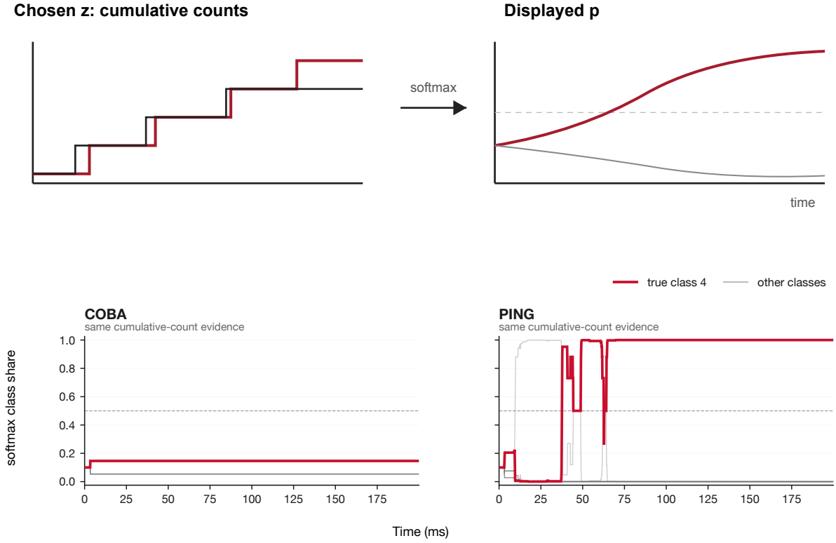
Figure 139: Ordinary softmax applied to cumulative spike counts. The measured mirror shows how an accumulating count margin becomes apparent confidence.
