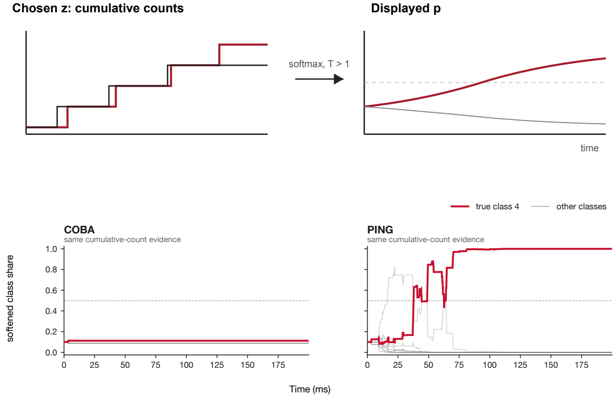
Figure 140: Temperature-softened softmax applied to the same counts. It differs from ordinary softmax only in temperature, isolating the effect of p .
