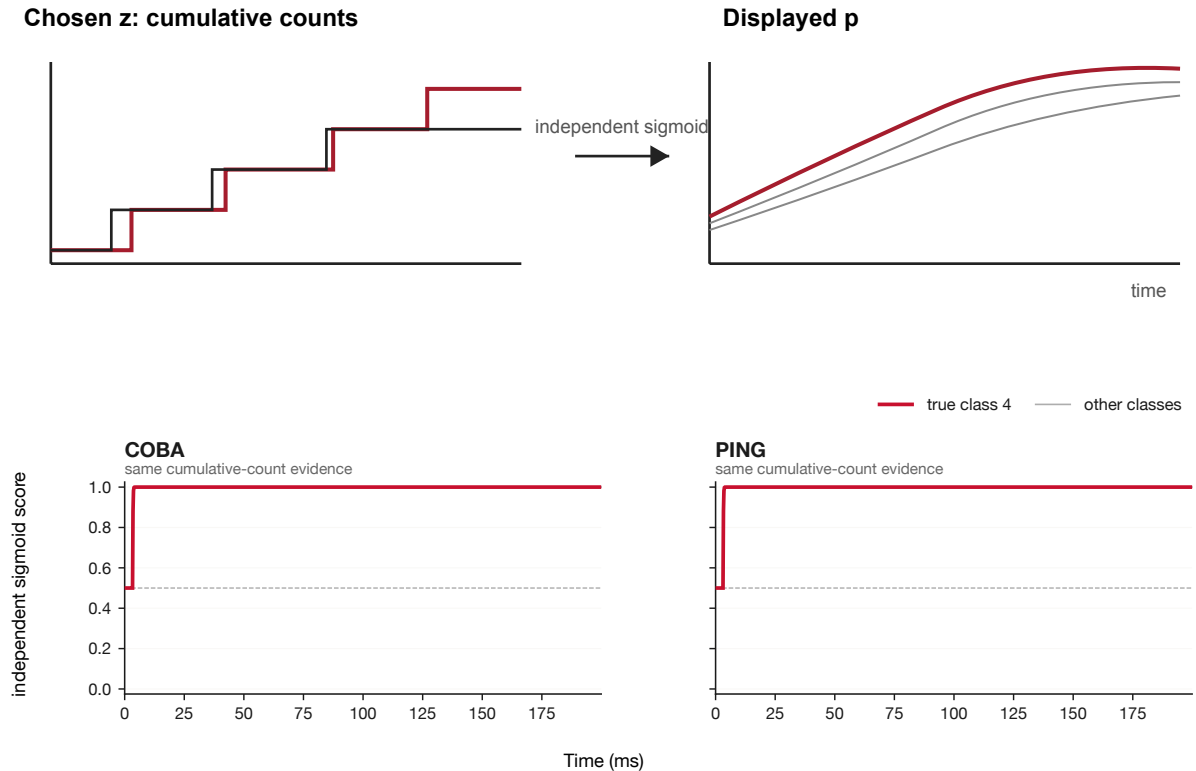
Figure 141: Independent sigmoid applied to cumulative spike counts. It retains the same z used by both softmax variants and reveals what is lost when classes no longer compete.
