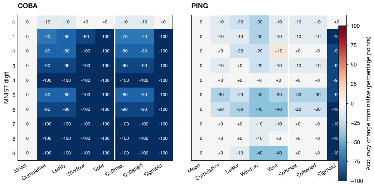
Figure 144: Class-specific change from native accuracy, in percentage points. The screen is balanced at ten images per digit, so each image changes its class cell by ten points.
