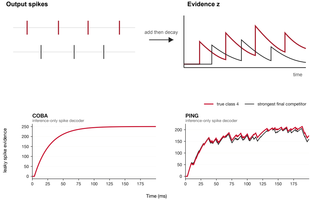
Figure 136: Leaky-count decoder. Spikes create upward steps and evidence decays smoothly between them, using the same leak factor for COBA and PING.
