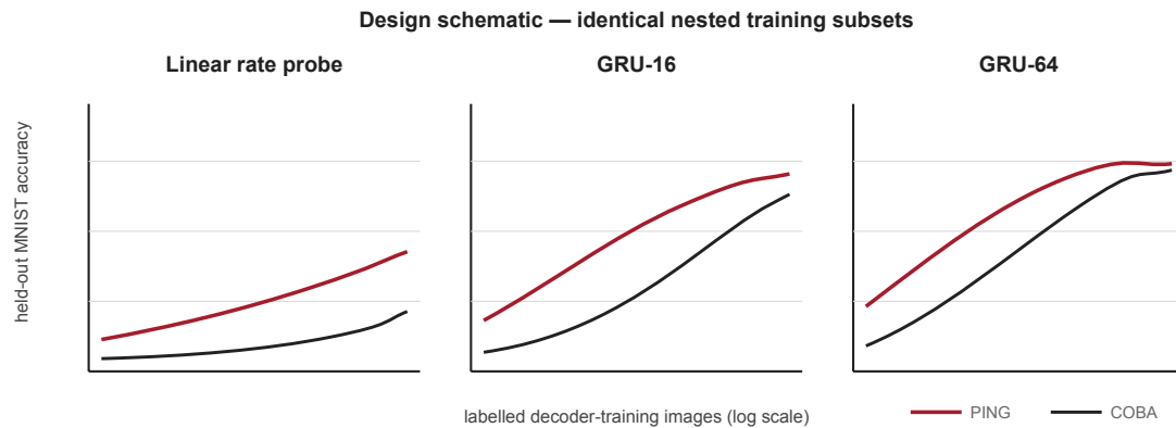
Figure 148: Design schematic for sample efficiency. Each decoder capacity receives the same nested labelled subsets for COBA and PING.
