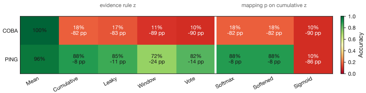
Figure 142: Decoder transfer screen. Each cell gives accuracy and, below it, the change from that network’s native mean-voltage decoder. The divider separates temporal evidence choices from mappings of the shared cumulative-count evidence.
