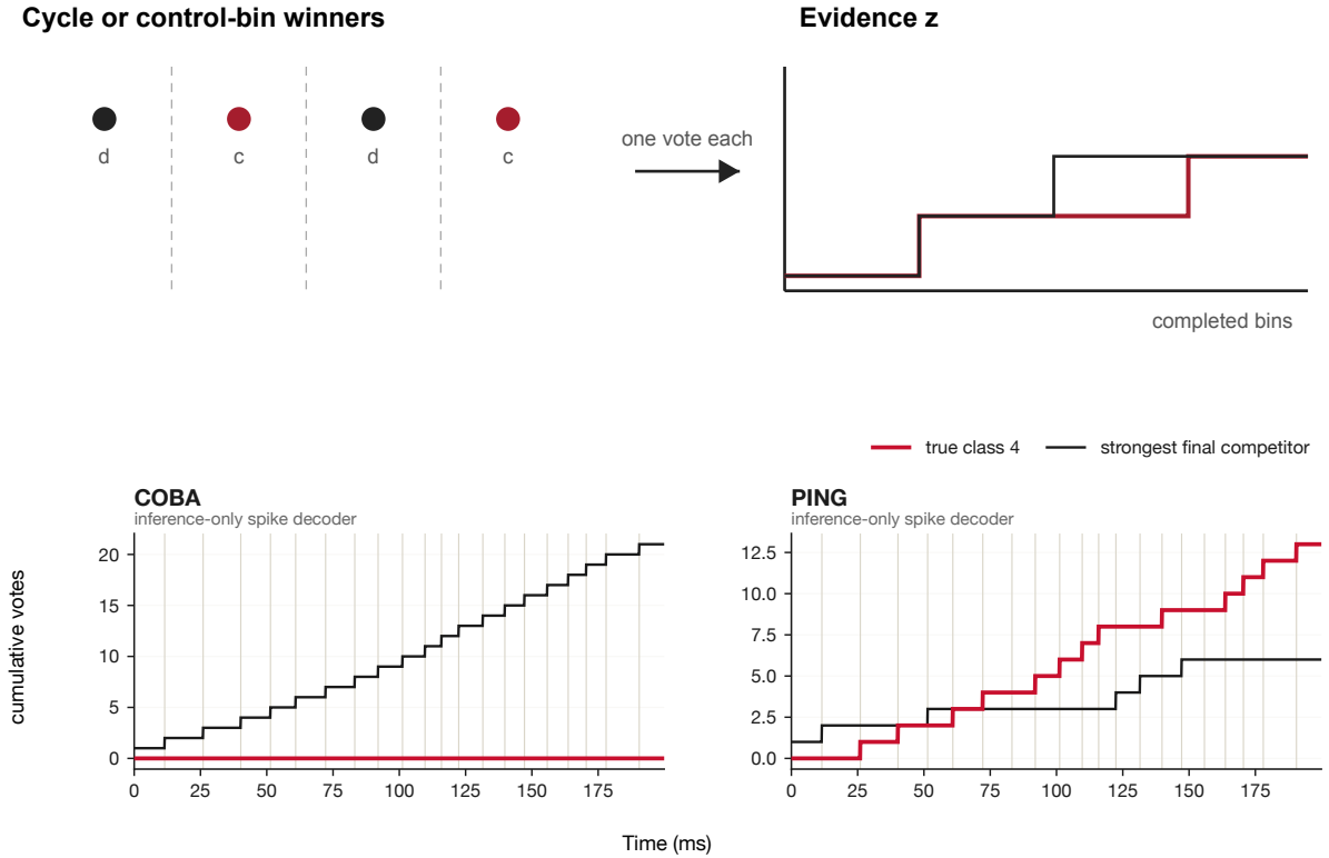
Figure 138: Cycle or matched-bin voting. Each interval names one winner before adding one vote. PING votes follow detected cycles and COBA votes use duration-matched controls.
