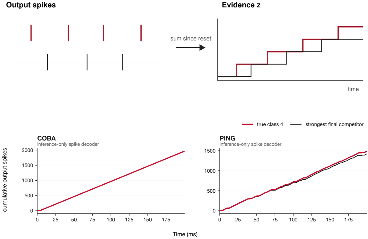
Figure 135: Cumulative-count decoder. Each output spike increments one class trace and no evidence decays; the staircase exposes early leads and later reversals.
