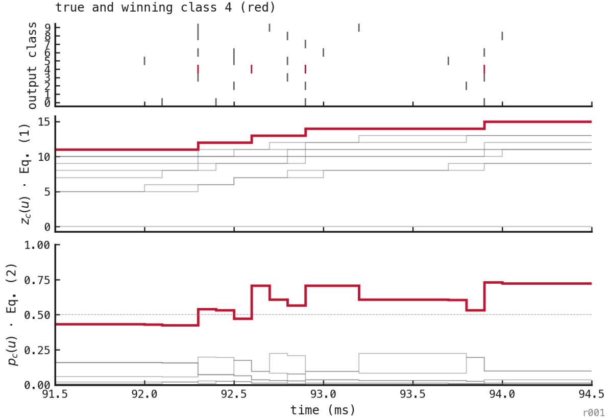
Figure 112: The 91.5–94.5 ms transition from Figure 1. Top: output-LIF spikes by class. Middle: cumulative counts z_{c(u)} from Equation 1. Bottom: p_{c(u)} from Equation 2. The true and winning class 4 is red; other classes are grey. The apparent jump in class evidence is produced by discrete count increments rather than by a continuous-valued readout.
