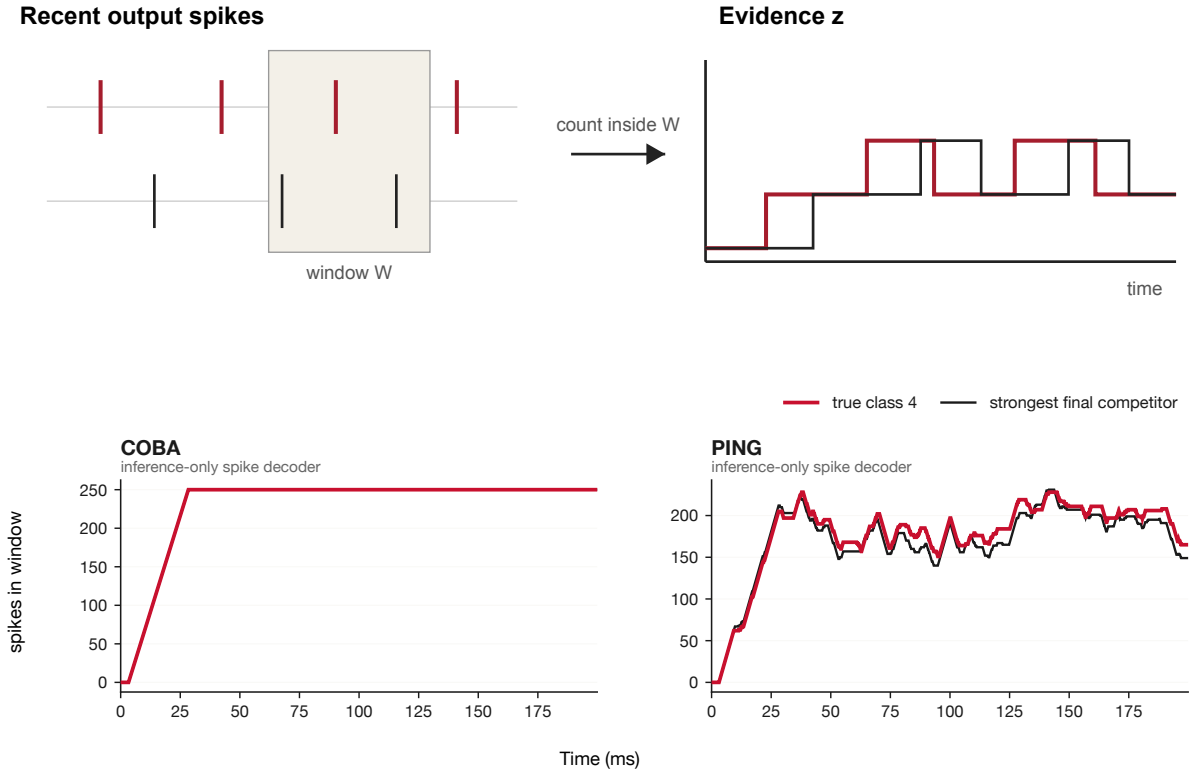
Figure 137: Sliding-window decoder. Evidence persists for 25 ms, then disappears abruptly when its spike leaves the window.
