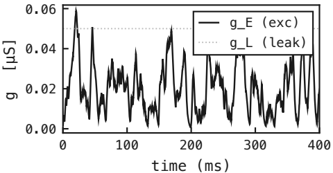
C0BA – no recurrent loop (ei-strength = 0) – E-neuron conductances (cell 57)
