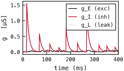
PING – recurrent loop active (ei-strength = 1.5) – E-neuron conductances (cell 547)
