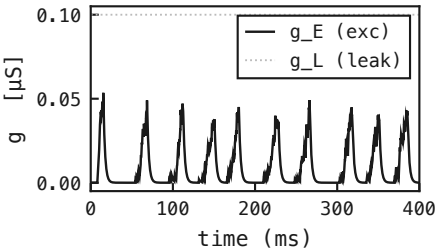
PING – recurrent loop active (ei-strength = 1.5) – I-neuron conductances (cell 81)
