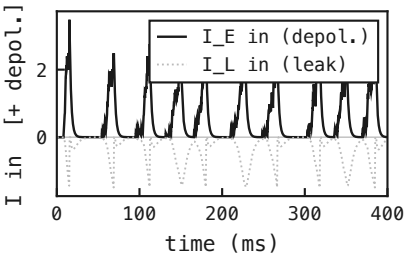
PING – recurrent loop active (ei-strength = 1.5) – I-neuron signed currents (cell 81)
