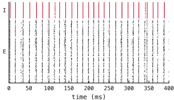
Same accuracy, fewer spikes ( \star = \theta_u off)
