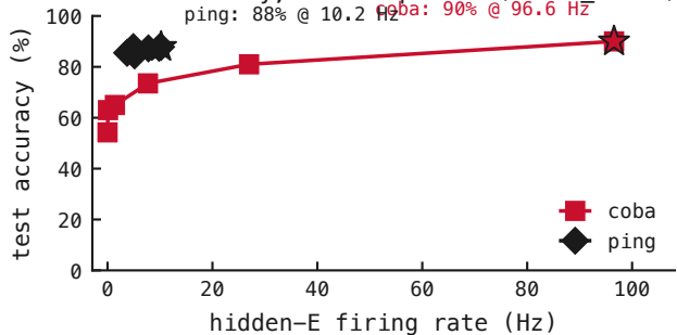
Same accuracy, fewer spikes ( \star = \theta_u off)
