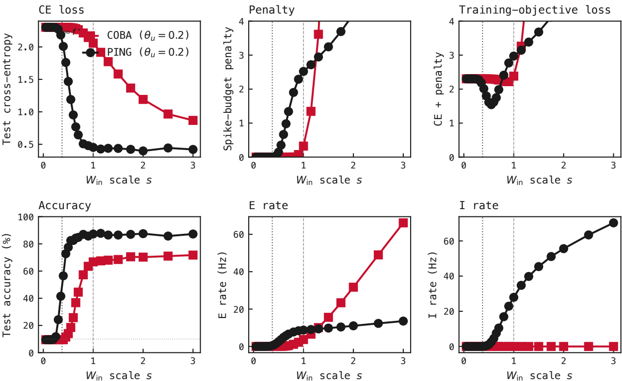
Inference-time W_{in} scale sweep on trained networks (dashed line = trained s=1 )
