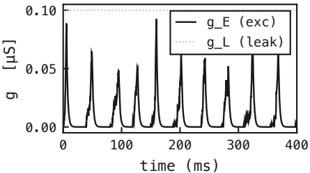
PING – recurrent loop active (ei-strength = 1.5) – I-neuron conductances (cell 3)
