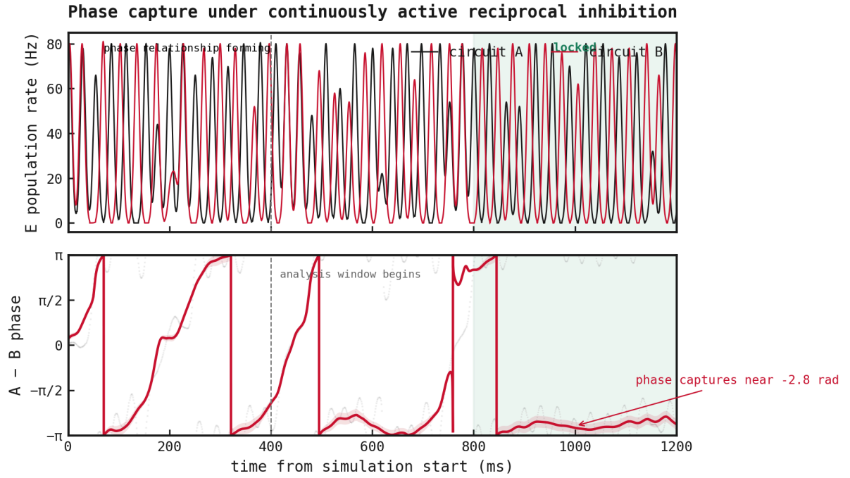
Figure 119: Phase capture during the first 1.2 s of the strength 0.2, intermediate-delay condition. Reciprocal coupling is active from the first timestep. The two population rhythms initially have an unstable relative phase; their circular phase difference then concentrates near -2.8 rad. This is phase locking, not zero-lag synchrony. The dashed line marks the registered transient exclusion and the green band highlights the capture interval. Full-window metrics and later phase slips remain included in the registered analysis.
