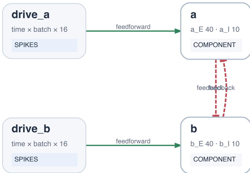
Figure 120: Representative reciprocal graph. Each inhibitory population sends a delayed GABA projection to the other circuit’s excitatory population; the two input nodes are independent.
