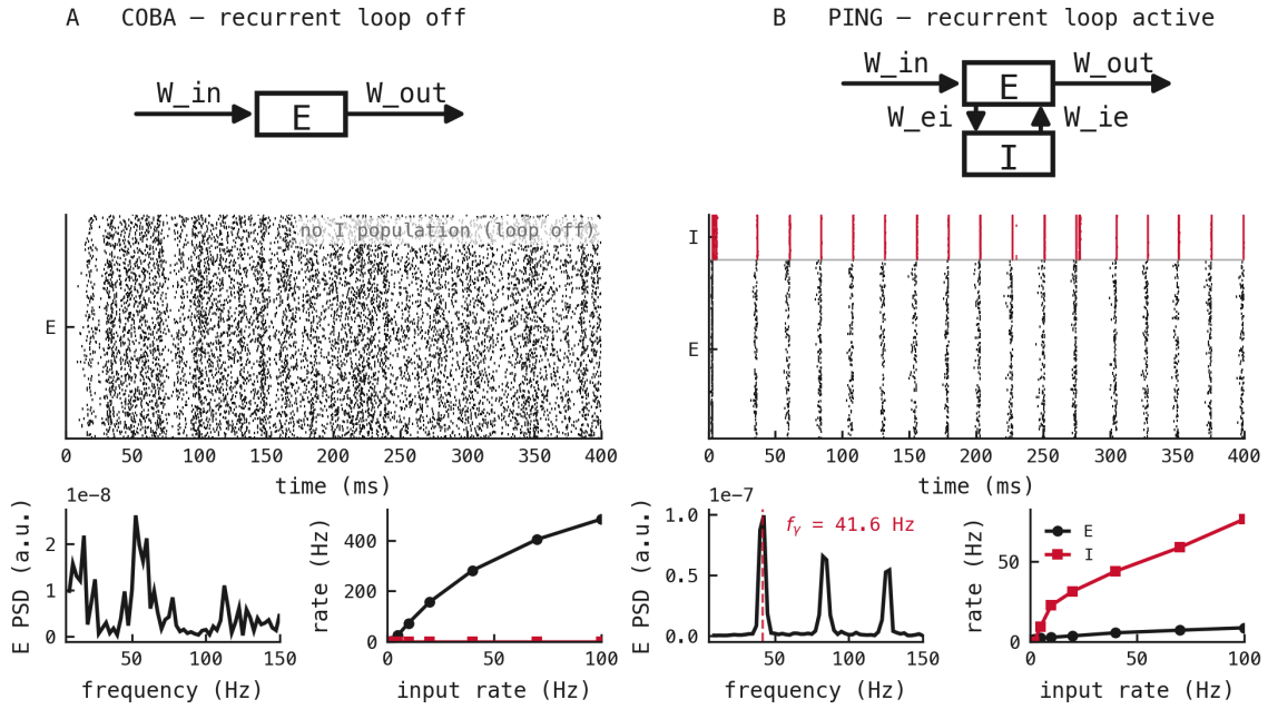
Figure 48: The architecture and its behaviour, off and on, on the same network. Each column carries its schematic on top — A COBA (input→ E →output, no I population) and B PING (the same plus the recurrent E \leftrightarrow I loop, W_{ei} down and W_{ie} up) — directly above the plots it produces. Below each schematic is one combined raster ( E black in the lower portion, I red in the upper portion — same axes, no gap) above a bottom row pairing the Welch PSD of the population-mean E trace with the free-running f - I curve (mean per-cell rate vs input rate, E black / I red; each column has its own y-axis — COBA runs to its \approx 400+ Hz ceiling, PING is on a smaller scale so its loop-clamped E and climbing I are legible). Rasters and spectra are on uniform Poisson input (400 ms) at per-condition rates (COBA 5 Hz, PING 45 Hz — see Methods); the f - I curves sweep that drive on the untrained network. All runs are at \Delta t = 0.1 ms. A — COBA ( ei-strength 0, loop off): asynchronous E firing, no I activity, no recurrent gamma peak, and an E f - I curve that climbs steeply with input rate and saturates toward the refractory ceiling. B — PING ( ei-strength 1.5, loop on): the I population fires a synchronous burst once per cycle and the E raster breaks into vertical bands (the I volley trails each E volley by the AMPA delay); the PSD carries a clean gamma peak (dashed red line; f_\gamma measured from this raster’s E -population PSD, marked on the plot); and its f - I shows the E rate held to single digits across the whole sweep (note the much smaller y-axis than COBA’s) while inhibition climbs — the loop’s dynamic-range compression. The single E \rightarrow I \rightarrow E loop is the only change: it converts asynchronous firing into a gamma rhythm and clamps the E rate.
