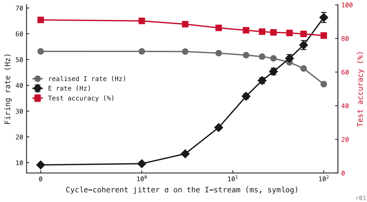
Figure 88: E rate (black diamonds) and accuracy (red squares) vs cycle-coherent jitter \sigma , three seeds. As \sigma grows the displaced bursts open wider gaps and the E rate climbs from baseline (9.1 Hz) past the full phase-shuffle level (25.9 Hz, the reference with within-burst structure destroyed) to 66.3 Hz by \sigma = 100 ms, with the sharpest rise near the predicted transition timescale \sigma = 1/f_\gamma \approx 22.8 ms; accuracy declines only gently, holding near 81.7%. The grey trace is the realised mean I rate: it holds within 3% of baseline through \sigma \approx 14 ms — where the E rate has already risen to 35.8 Hz — then droops to 40.5 Hz (24% below baseline) by \sigma = 100 ms, as the finite trial window truncates the most-displaced bursts. The strict same-mean-inhibition comparison is read at the smaller \sigma , where the rate is matched and the E rise is already unambiguous.
