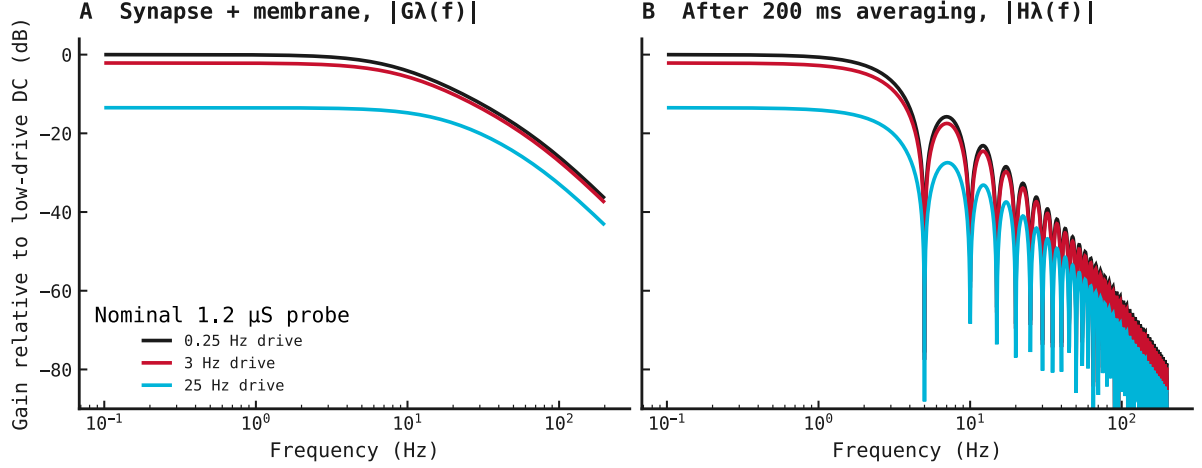
Figure 120: Analytically calculated linearized frequency response at the nominal 1.2 \mu\text{S} probe. The functions take modulation frequency, mean input rate, and probe conductance; they contain no simulated traces. Frequency is a small sinusoidal rate modulation around 0.25, 3, or 25 Hz. Panel A evaluates Equation 13 ( G_\lambda ) from 0.1–200 Hz, with \omega = 2\pi \frac{f}{1000} rad/ms. Gain is
