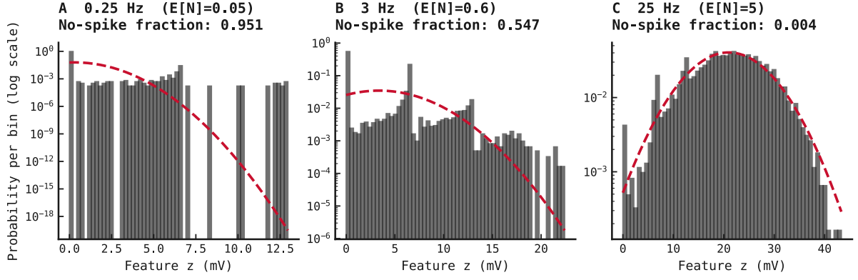
Figure 119: Transition from sparse shot noise toward a Gaussian-like feature distribution. Each panel contains 6144 recorded z values: 2048 simulations \times three seeds for pixel intensity 255 and the nominal 1.2 \mu\text{S} probe. Bars show empirical probability per bin on a logarithmic axis; the red dashed curve is a Gaussian with the same empirical mean and SD. Panel A, at 0.25 Hz, is dominated by no-spike presentations and separated responses to rare spike counts and times. Panel B, at 3 Hz, remains strongly non-Gaussian because more than half of presentations contain no spike. Panel C, at 25 Hz, contains about five expected spikes per presentation; overlapping filtered responses form a much smoother distribution that approaches the matched Gaussian, while conductance nonlinearity and finite-window timing leave visible deviations.
