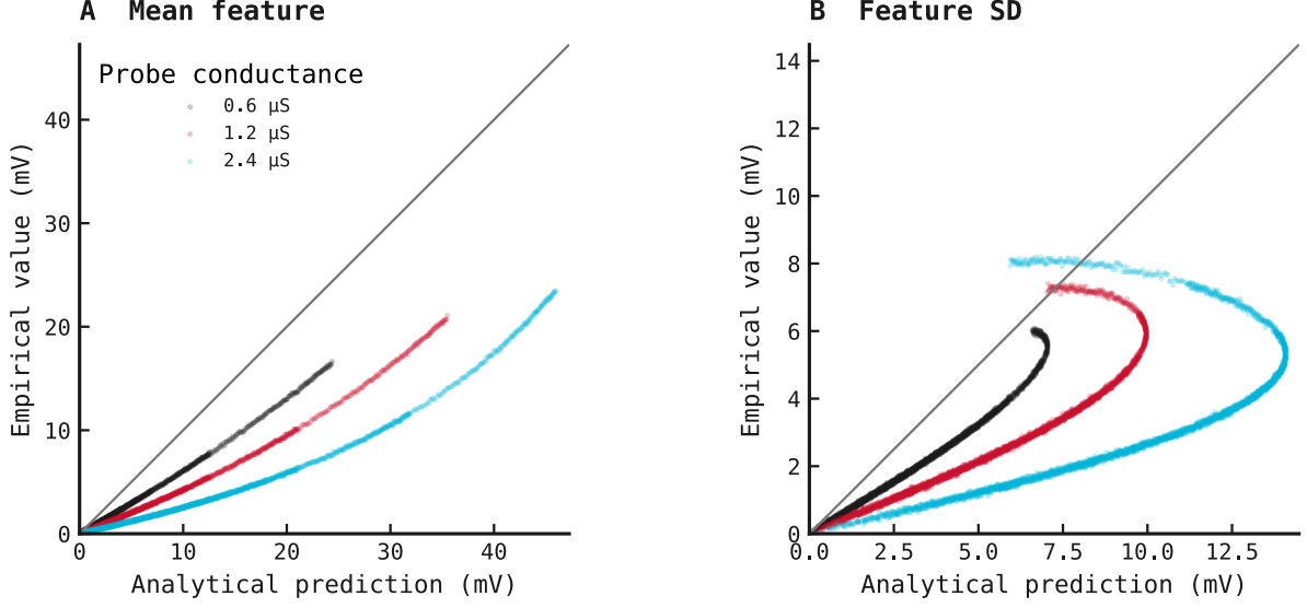
Figure 121: Operating-point linearized predictions versus empirical response moments. Each point is one rate–intensity condition; colour denotes probe conductance, and empirical moments pool draws across three seeds. Panel A compares the predicted mean of z from Equation 12a ( \mu_{\text{linear}(z)} ) with the empirical mean of z . Panel B compares the predicted SD of z , \sqrt{\text{Var}_{\text{linear}(z)}} from Equation 18, with the empirical SD of z . The diagonal marks equality. Mean ordering is preserved (Pearson r = 0.951 ), but the median prediction is 2.52-fold larger. SD agreement is weaker ( r = 0.741 ), with median 2.245-fold overprediction. Points lie mainly below equality because the stationary linearization omits the start-from-rest transient, finite-window nonstationarity, discrete input, and conductance fluctuations.
