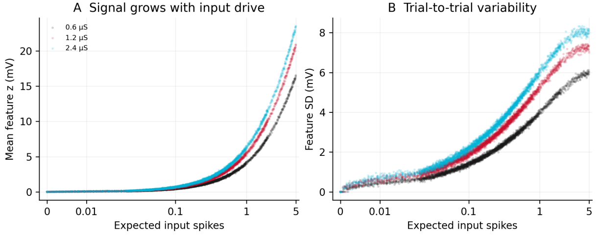
Figure 118: Mean and variability of the simulated single-pixel feature. We evaluated 9,216 conditions: 256 pixel intensities \times 12 encoding rates \times three probe conductances. For each condition, we selected 512 simulations from each of three independent random seeds, giving 1536 values of feature z . Each point in Panel A is the mean of those 1536 values; the corresponding point in Panel B is their standard deviation. Thus, each panel contains 9,216 points. The 512 simulations per seed were chosen as a practical descriptive subset of the available simulations, not through a statistical convergence test. The horizontal axis is the expected number of input spikes during the 200 ms presentation: encoding rate \times normalized pixel intensity \times 0.2 s. Colour identifies probe conductance. Mean response increases with expected spike count. Variability initially rises as spike counts and times diversify, then can plateau or fall when averaging, shunting, and voltage saturation limit additional excursions.
