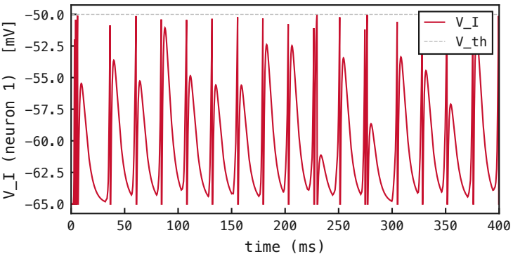
PING · I-neuron membrane voltage
