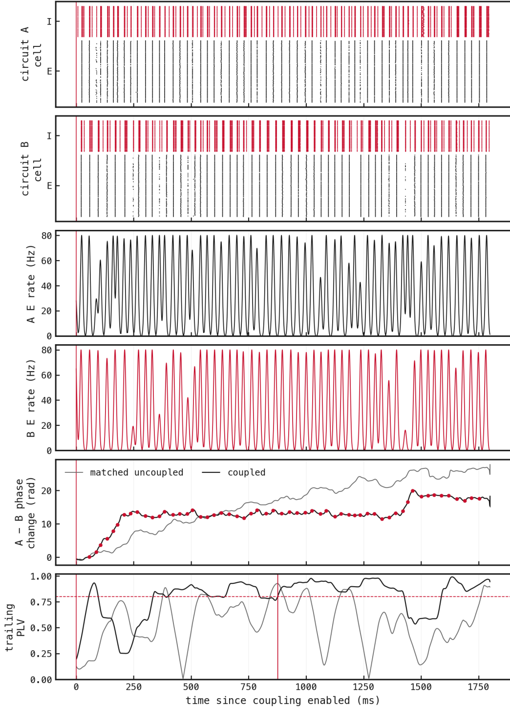
Figure 2: One continuous coupled trajectory from an already mature checkpoint selected at 3.141 rad separation. Reciprocal E→I weight 0.18 and delay 10 ms are enabled at 0 ms; nothing else is reset. The first two panels show fixed samples of 100 E and 50 I neurons from circuits A and B. The next two show their full-population E rates on a common scale without overlap. The final two panels directly compare unwrapped A-minus-B phase and 150 ms trailing PLV. Coupling arrests phase drift for many cycles and crosses the sustained-250-ms capture gate at 876 ms; the light identical-state control continues drifting. The later coupled phase jump and PLV trough are shown, not cropped: this seed exhibits metastable capture with one late slip, not permanent phase locking.
