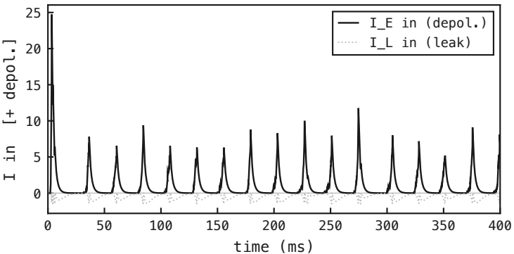
PING · I-neuron signed currents (cell 1)
