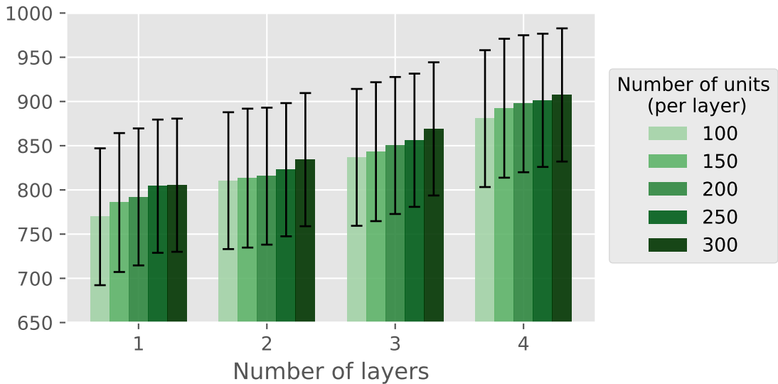
Peak memory during prediction (MiB)
