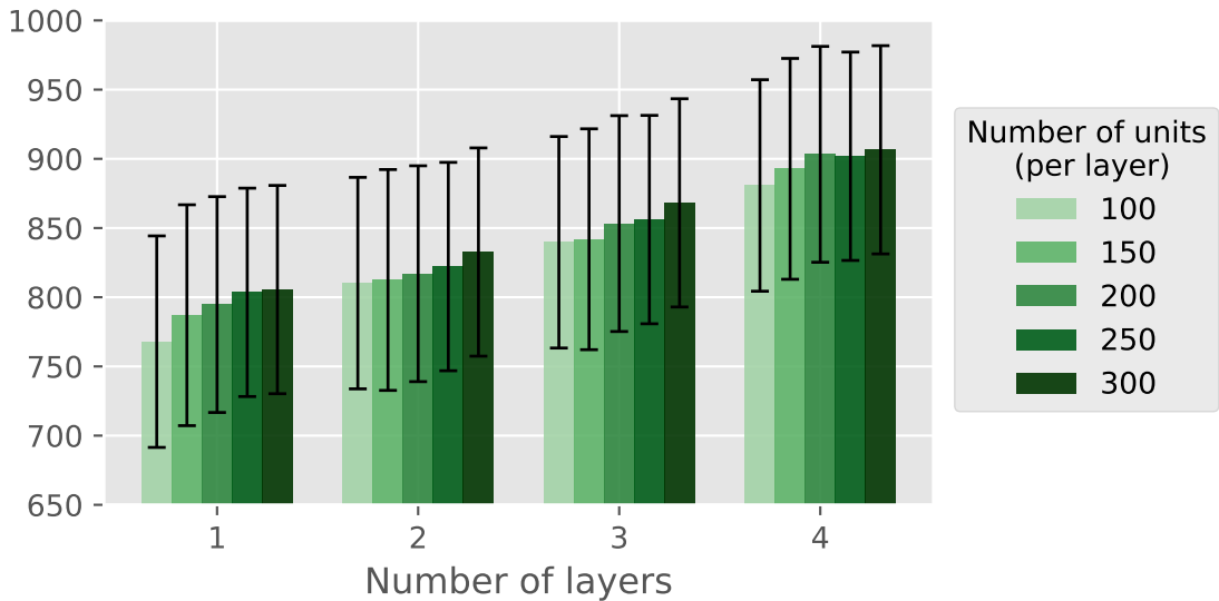
Peak memory during fitting (MiB)
