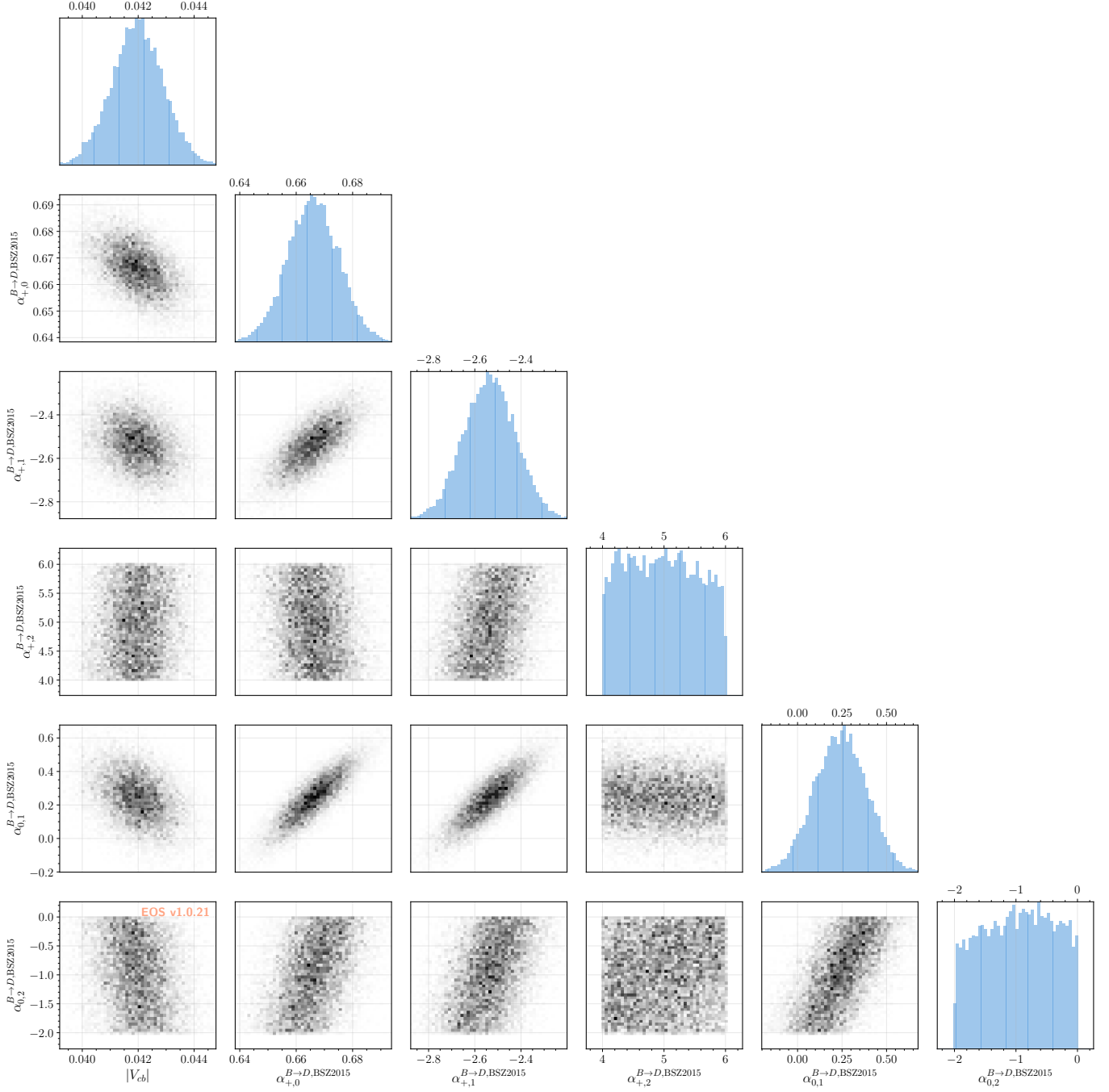
Figure 1: Corner plot of the marginal posterior densities for posterior CKM.
