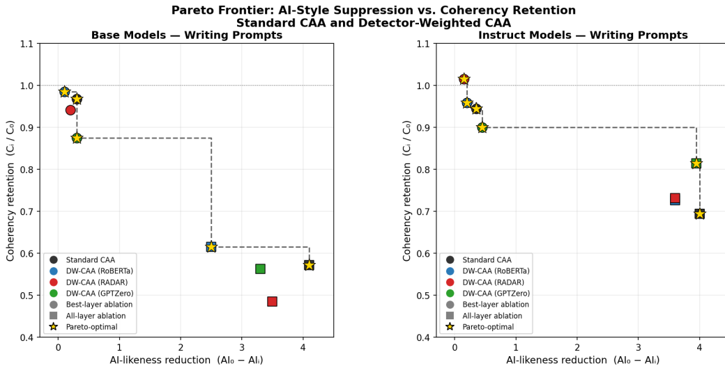
Figure 9: Pareto frontier for the eight ablation conditions in Table 3 on writing prompts, for QWEN2.5-3B (left) and QWEN2.5-3B-INSTRUCT (right). Each point is one ablation condition. Dashed line marks the Pareto frontier. The instruct frontier sits consistently higher than the base frontier, reflecting a more favorable tradeoff across all methods.
