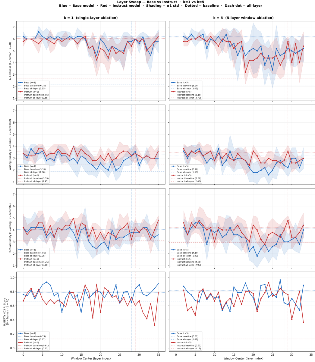
Figure 8: Layer sweep ablation results across all 36 layers for QWEN2.5-3B (blue) and QWEN2.5-3B-INSTRUCT (red), with k = 1 (left column) and k = 5 (right column). The top rows show LLM-judge metrics (AI-likeness, writing quality, factual quality) collected alongside the primary RoBERTa HC3 AI score (bottom row). Dotted horizontal lines mark the unablated baseline; dash-dot lines mark all-layer ablation. Shaded regions are \pm 1 SD. The best-classifying layer (28-29, gray dashed vertical line) consistently produces near-zero change across all metrics, while the causal generation region at middle layers produces the largest reductions in AI-likeness.
