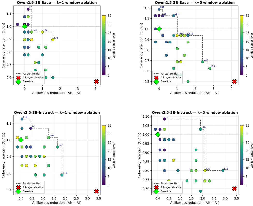
Figure 10: Pareto frontier for the layer sweep across all 36 window positions, for k = 1 and k = 5 , on writing prompts. k = 5 windows consistently Pareto-dominate k = 1 windows. The instruct model frontier sits above the base model frontier at every suppression level.
