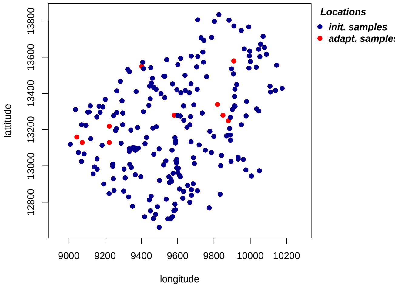
Existing design plus adaptive samples
