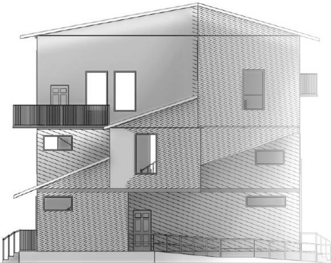
South Elevation
