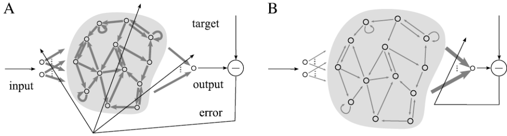
Figure 2.7: Comparison of B) RC vs A) traditional RNN, the bold arrows are weights that change during training [19]
