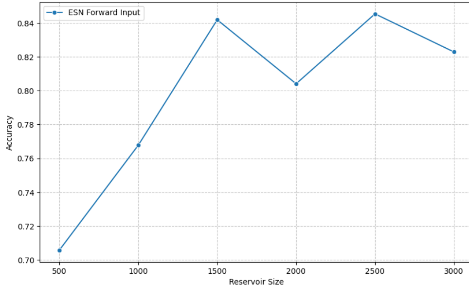
Figure 5.2: Network accuracy vs. reservoir size for 50 epochs runs.
