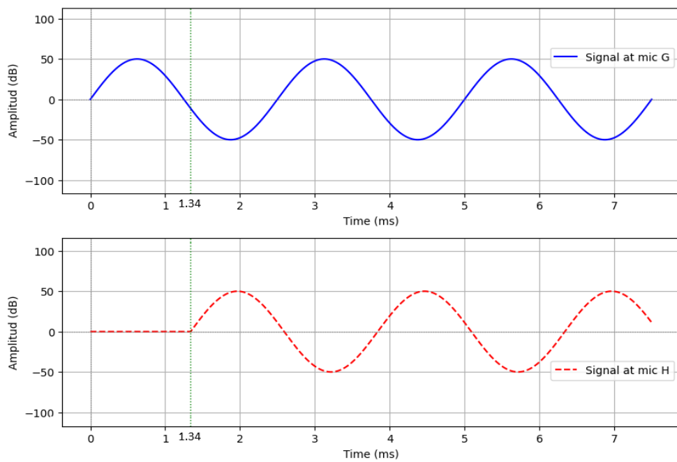
Figure 5.7: Acoustic waveforms at 400 Hz captured by the microphones located at points G and H.
