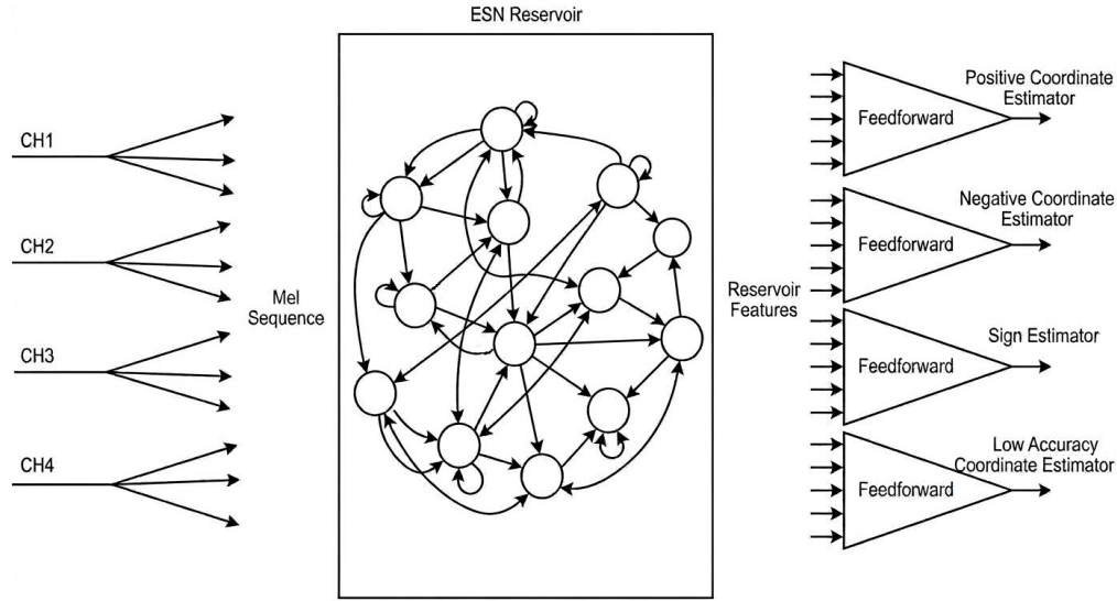
Figure 5.4: Multihead Network architecture for the ESN Estimator.
