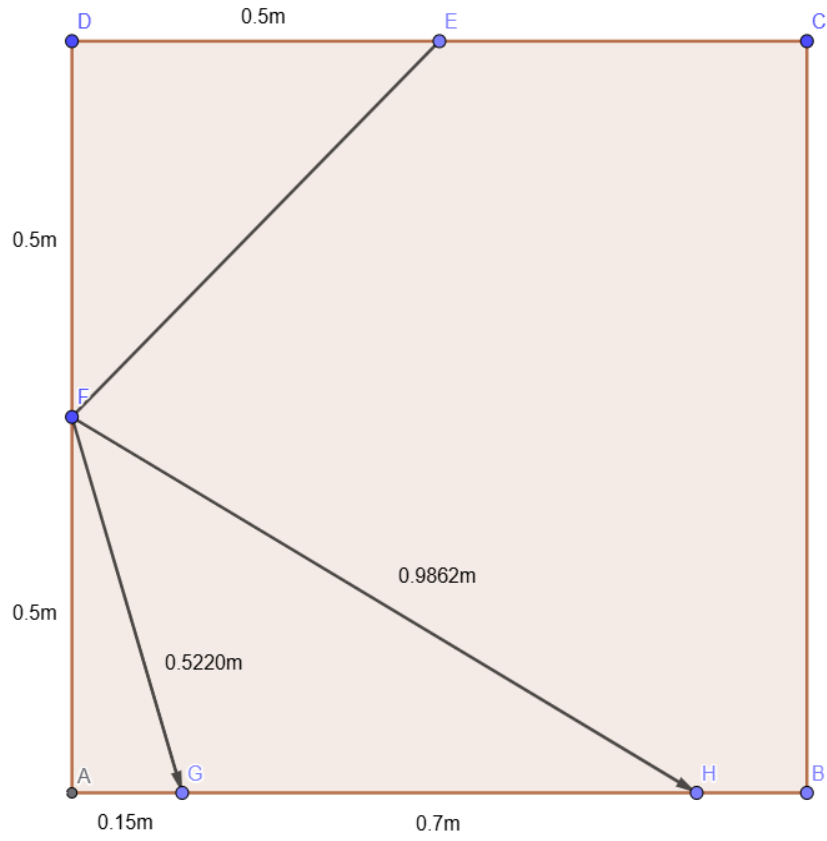
Figure 5.6: Geometric layout of the measurement box illustrating the acoustic path from the speaker located at E to the microphones positioned at G and H.
