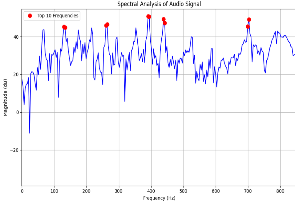
Figure 5.5: Frequency response of the stimulus signal showing the top 10 spectral components with the highest magnitude.
