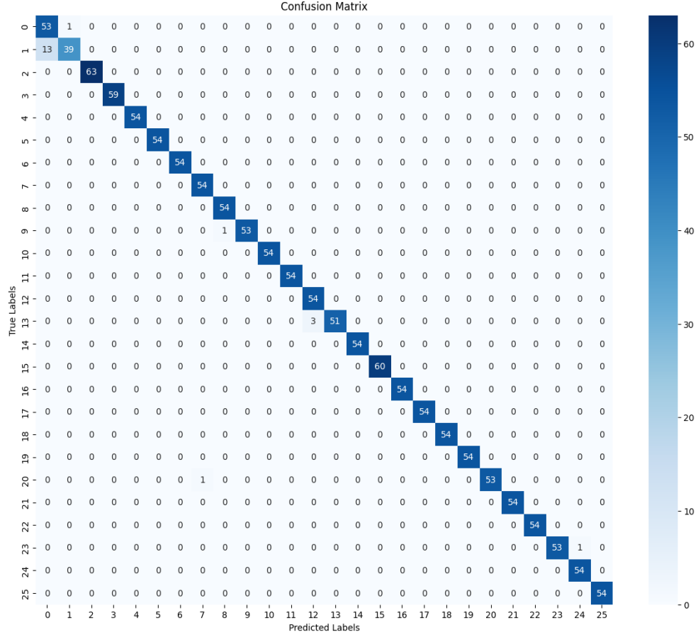
Figure 6.1: Confusion matrix for CNN acoustic location classification on test set.
