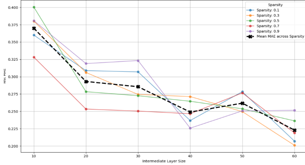
Figure 5.3: Test MAE as a function of Intermediate Hidden Layer Size for different Sparsity values
