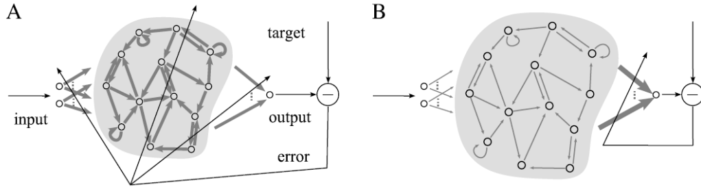
Figure 2.7: Comparison of B) RC vs A) traditional RNN, the bold arrows are weights that change during training [?]
