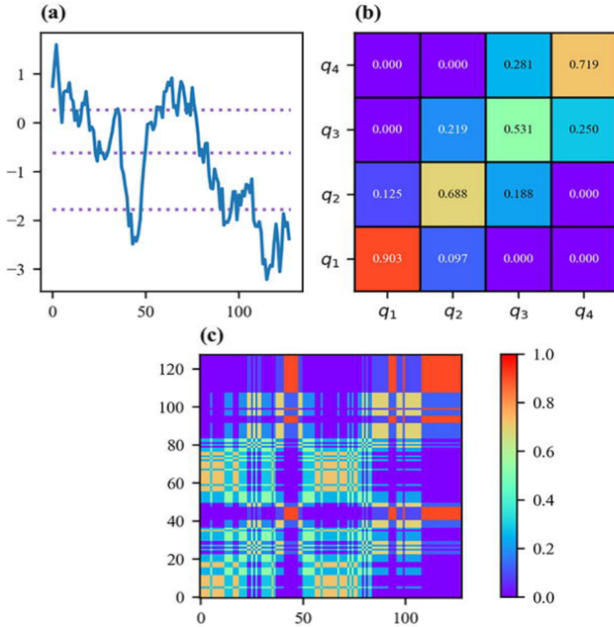
Figure 2.3: Summarized process to build a Markov Transition Field [? ]
