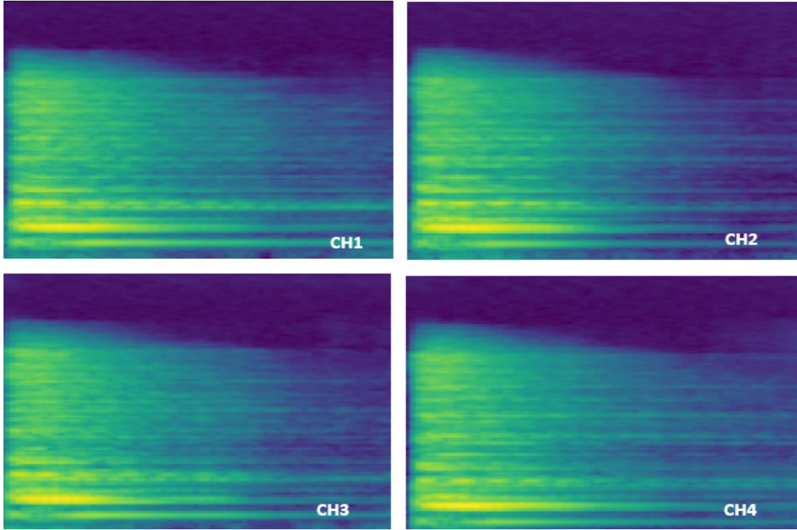
Figure 5.1: Log-Mel spectrograms correspondig of the four channels of signals captured at session 1, location X=22.8, Y=-0.94 , Z=-9.43 and orientation 50 degrees.
