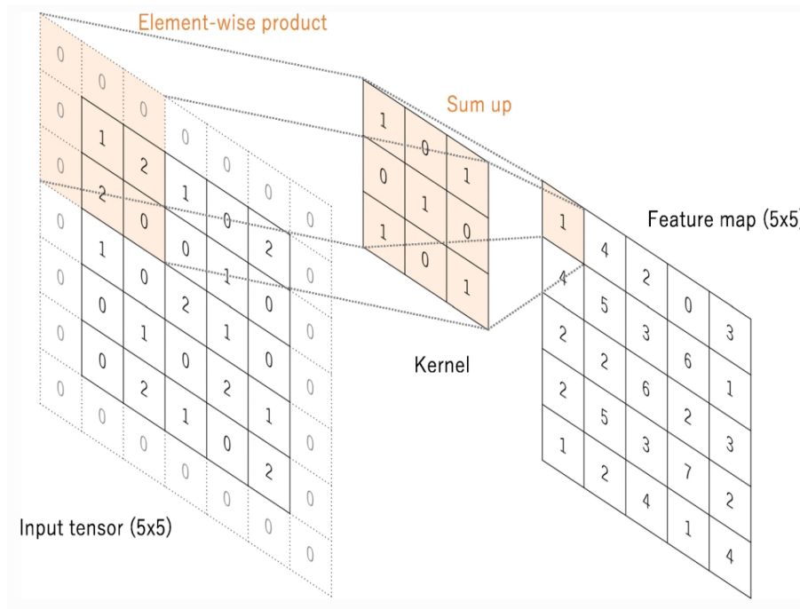
Figure 2.4: Convolution operation over a tensor of 5x5 with zero padding and a stride of 1, resulting in a feature map of 5x5 [? ]
