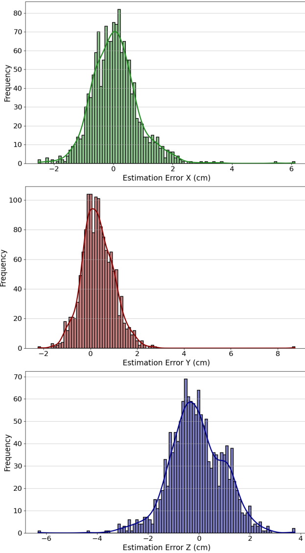
Fig. 5: Histograms of the estimation errors for each coordinate with the test set after training.
