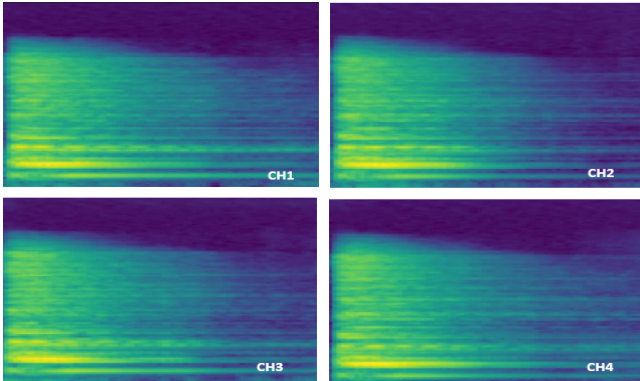
Fig. 3: Log-Mel spectrograms corresponding to the four channels of signals captured at session 1, location X=22.8 , Y=-0.94 , Z=-9.43 and orientation 50 degrees.
