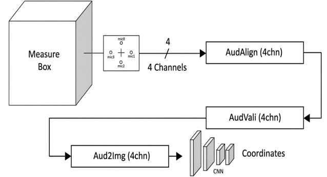
Fig. 4: Diagram of the audio data processing pipe for the estimator.
