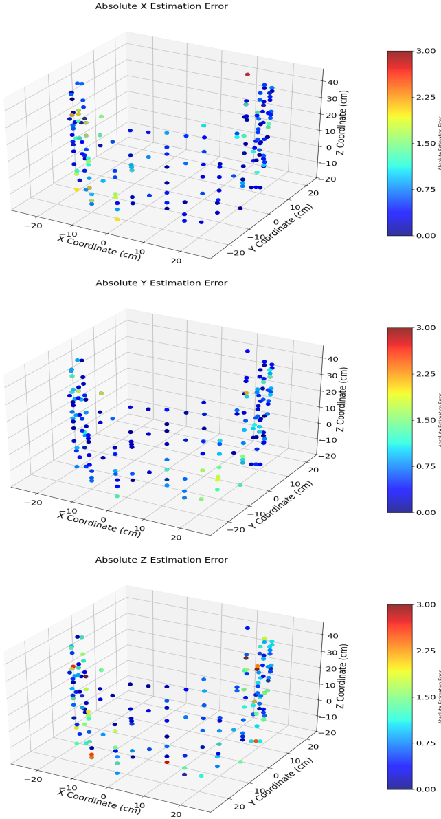
Fig. 7: Absolute value of the error estimation for the three networks as function of the three coordinates X, Y and Z
