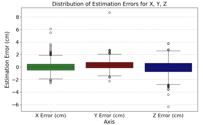
Fig. 6: Box-plot of estimation error for the three coordinates X, Y and Z
