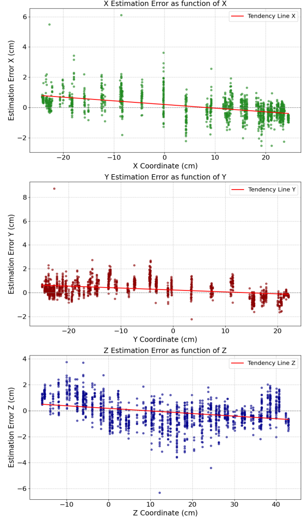
Fig. 8: Estimation errors along the three coordinates X, Y and Z as function of the corresponding coordinate value.
