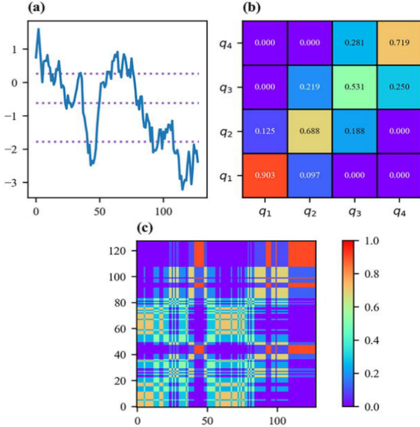
Figure 2.3: Summarized process to build a Markov Transition Field [13]
