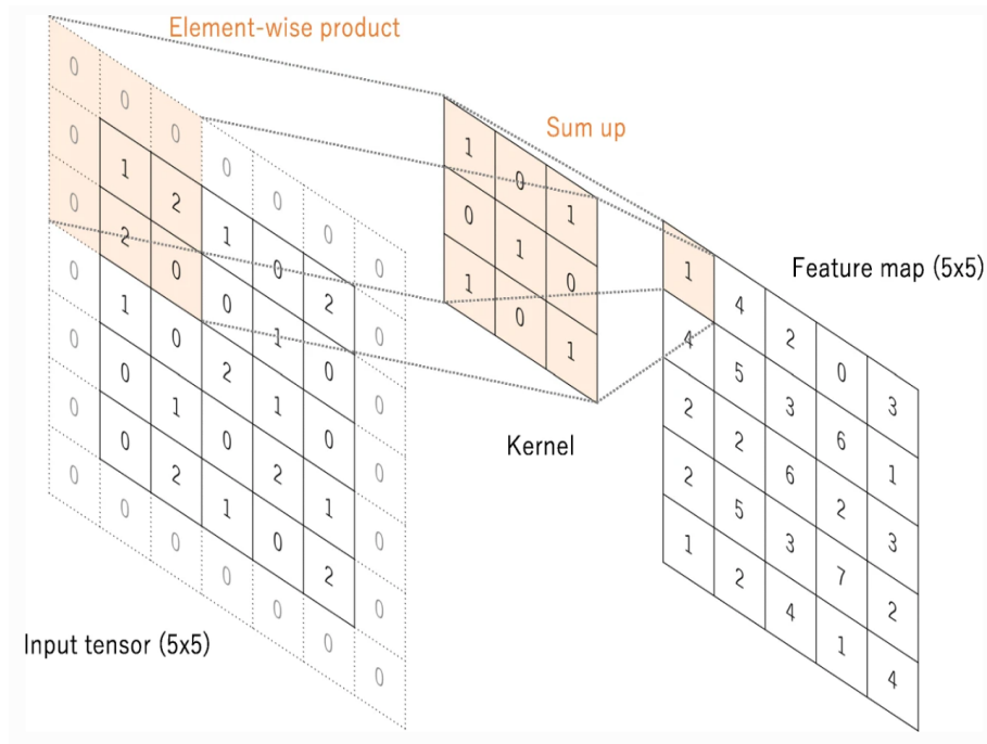
Figure 2.4: Convolution operation over a tensor of 5x5 with zero padding and a stride of 1, resulting in a feature map of 5x5 [47]
