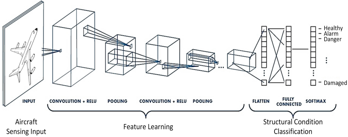
Figure 2.6: Structure of Convolutional Neural Network for aircraft structural health monitoring [36]
