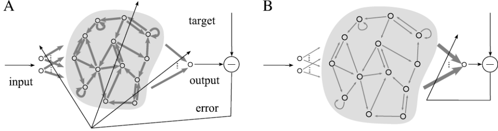
Figure 2.7: Comparison of B) RC vs A) traditional RNN, the bold arrows are weights that change during training [20]
