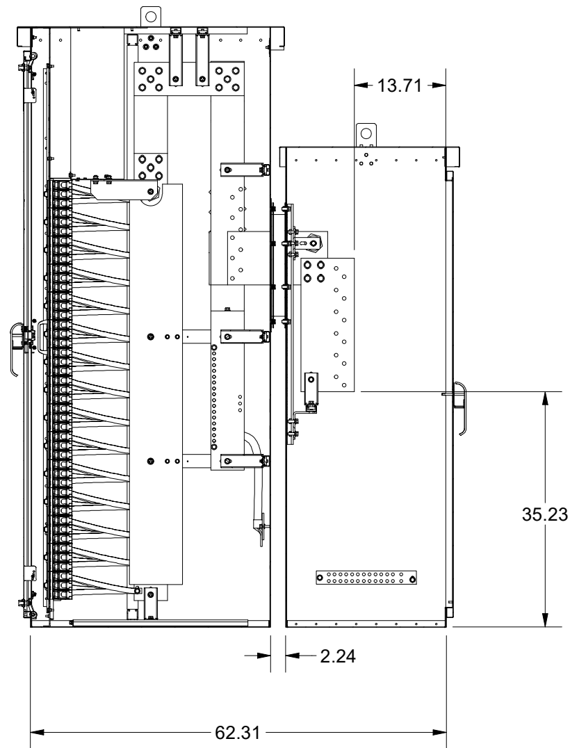
SECTION E-E
