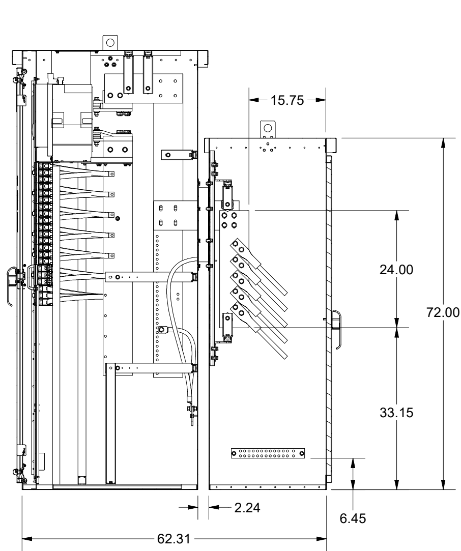
SECTION E-E
