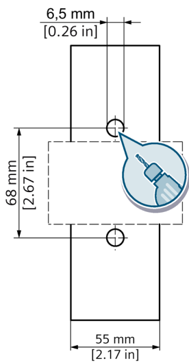
3WA9111-0AA31
