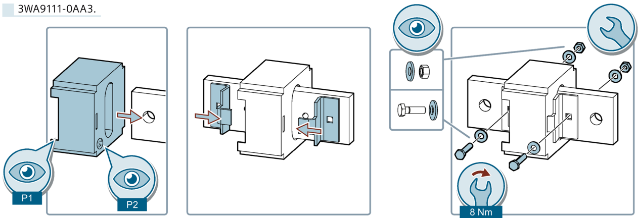
3WA9111-0AA31
