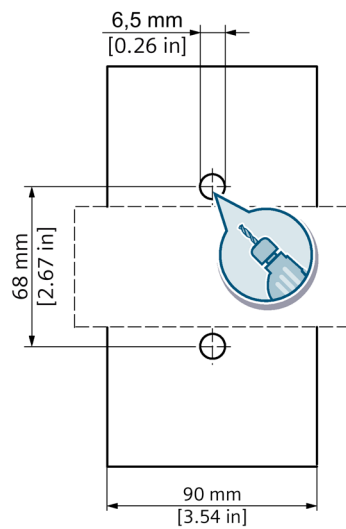
3WA9111-0AA32
