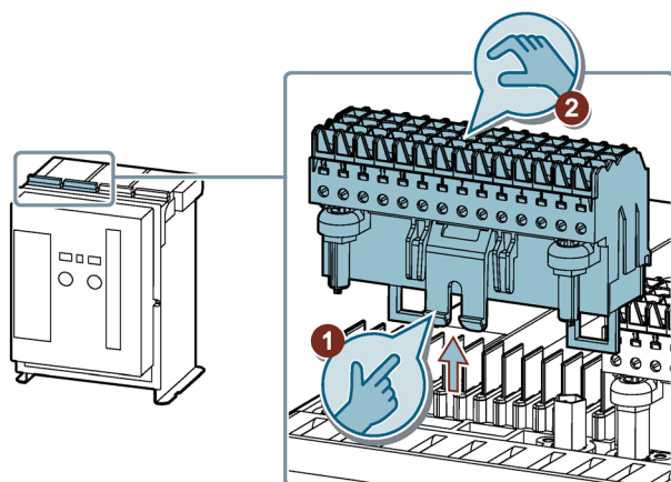
3WA9111-0BA3. 3WA9111-0BA43
