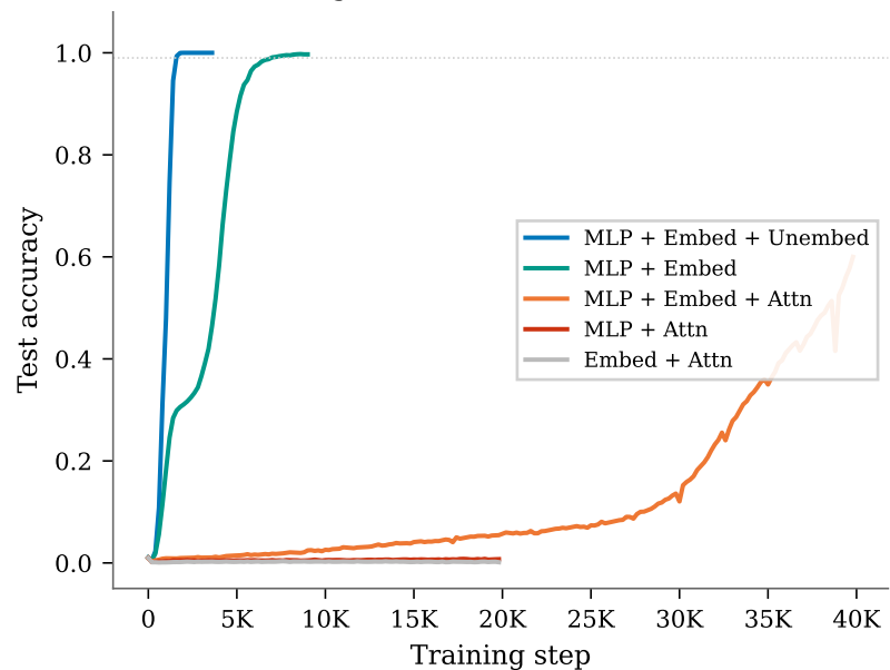
(b) Learning curves for each combination
