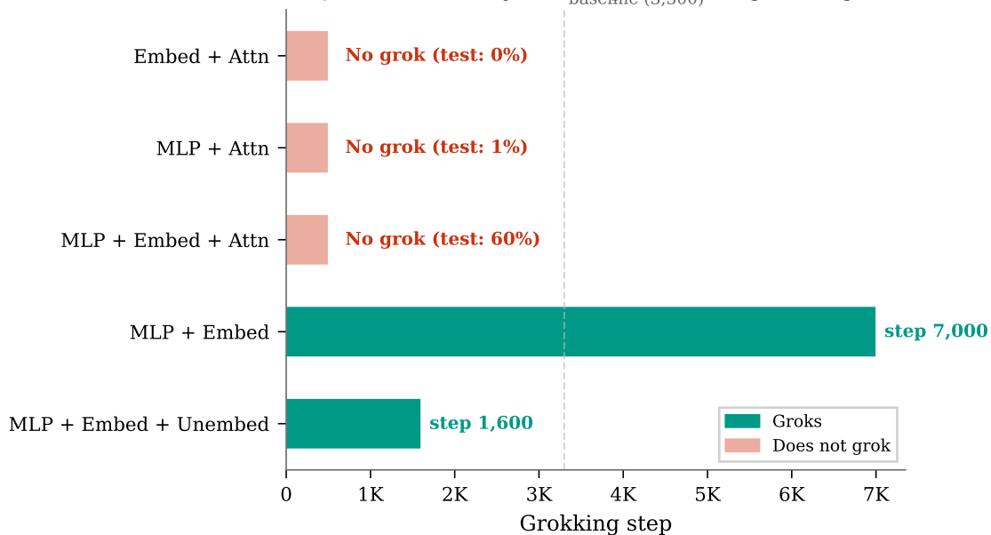
(a) Joint sufficiency: which pairs drive grokking?
