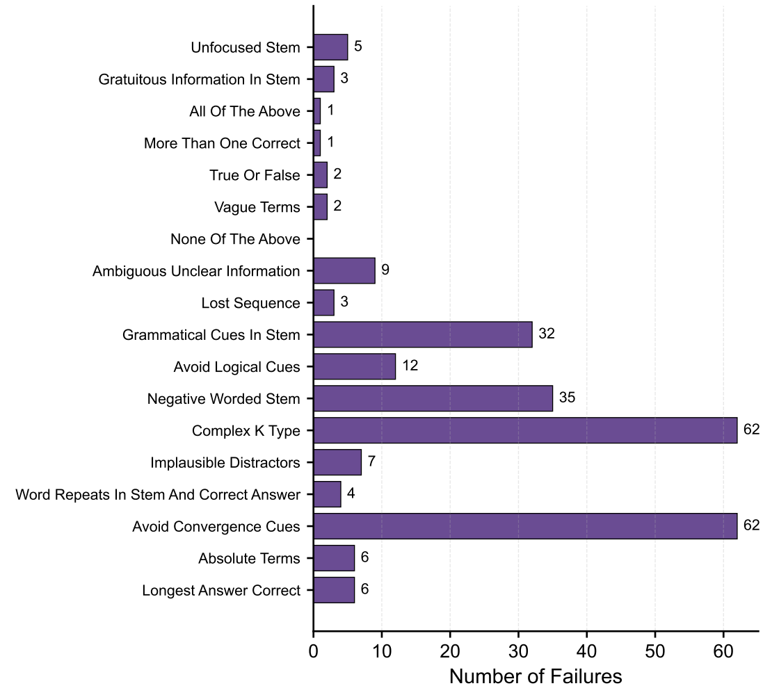
SME-Written Questions: Failures by Criterion
