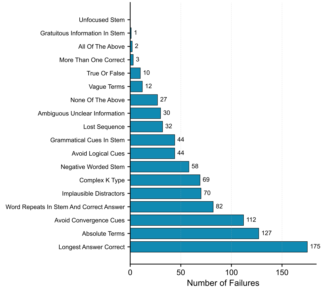
AI-Generated Questions: Failures by Criterion
