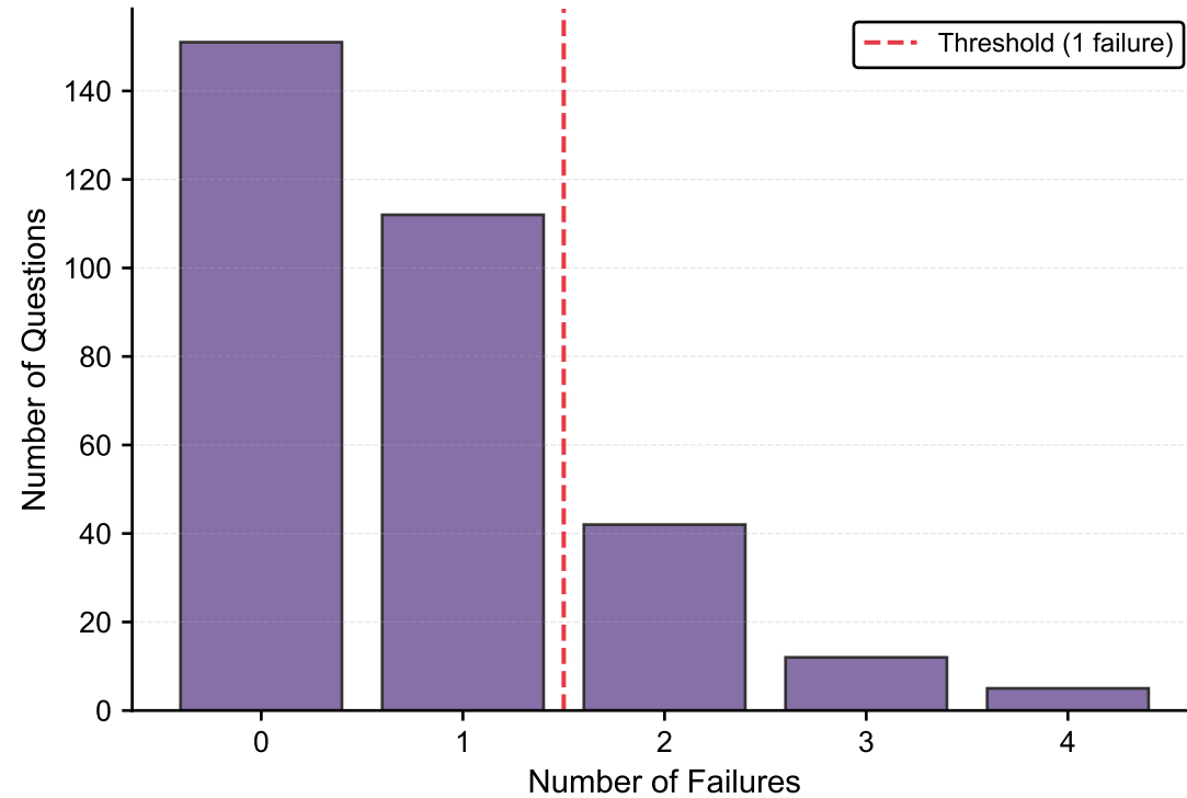
SME-Written Questions: Failure Distribution
