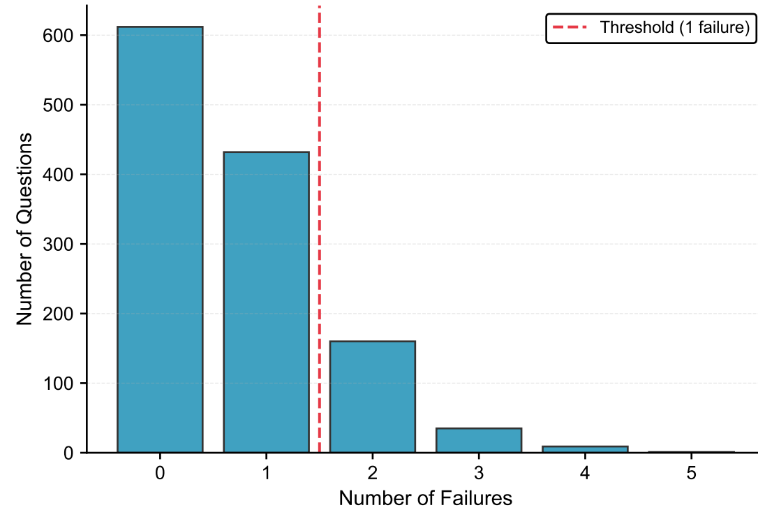
AI-Generated Questions: Failure Distribution
