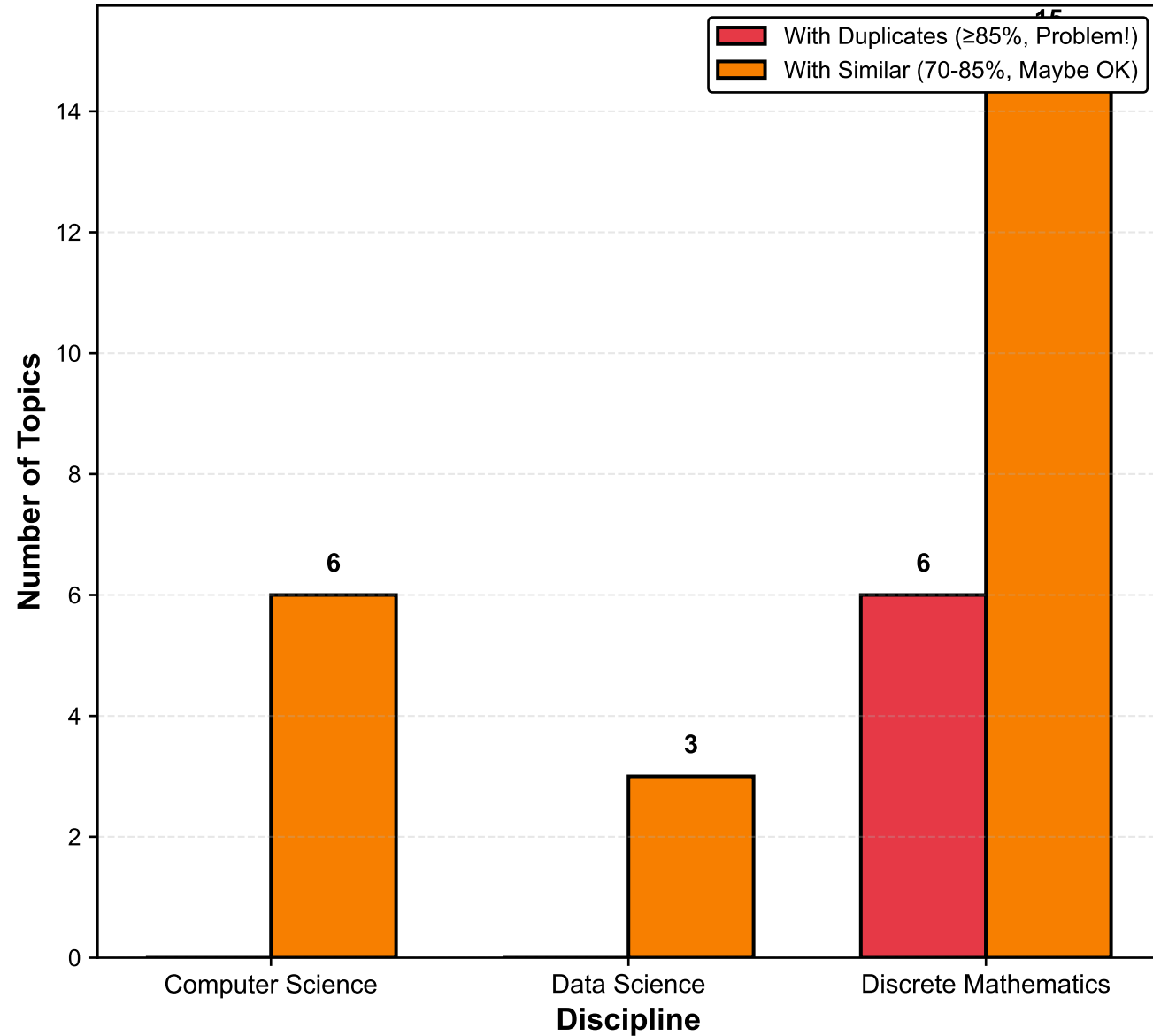
Within-Run Analysis: Duplicates vs Similar Questions (Duplicates = Problem | Similar = Potentially Acceptable)
