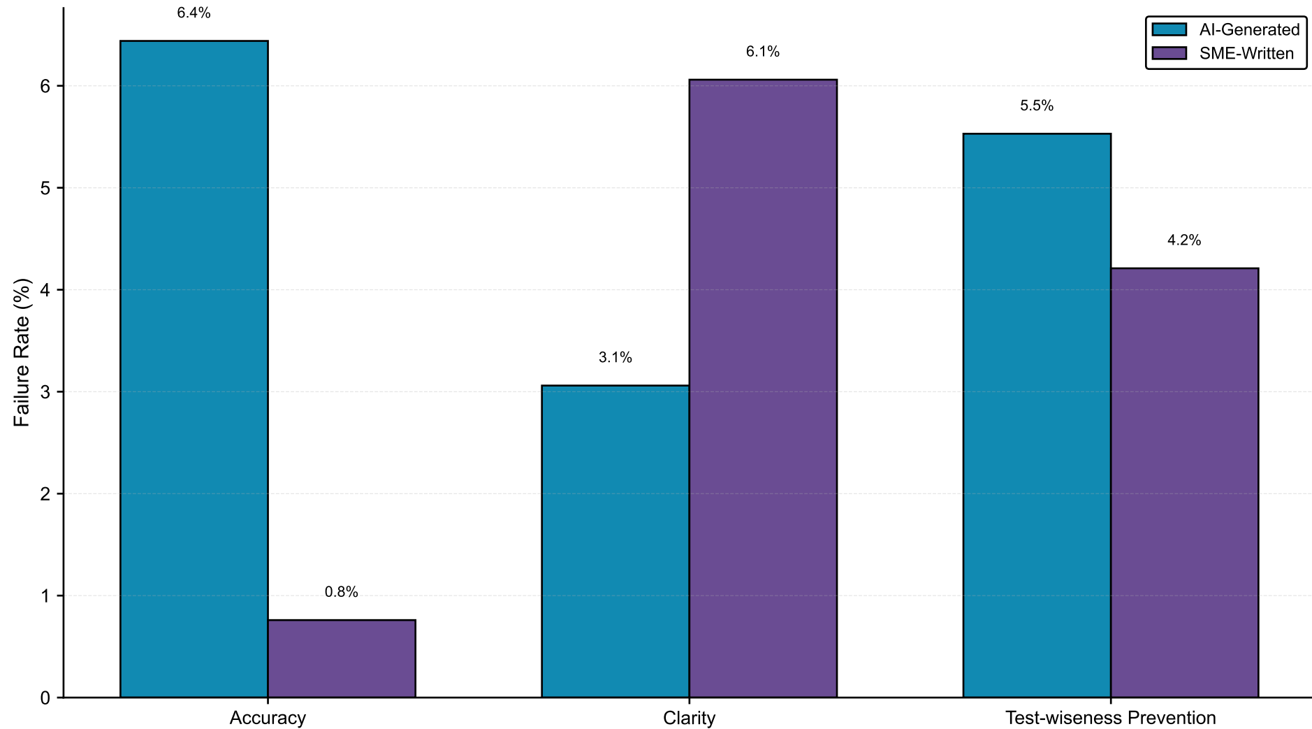
Discrete Mathematics: SAQUET Failure Rate by Category
