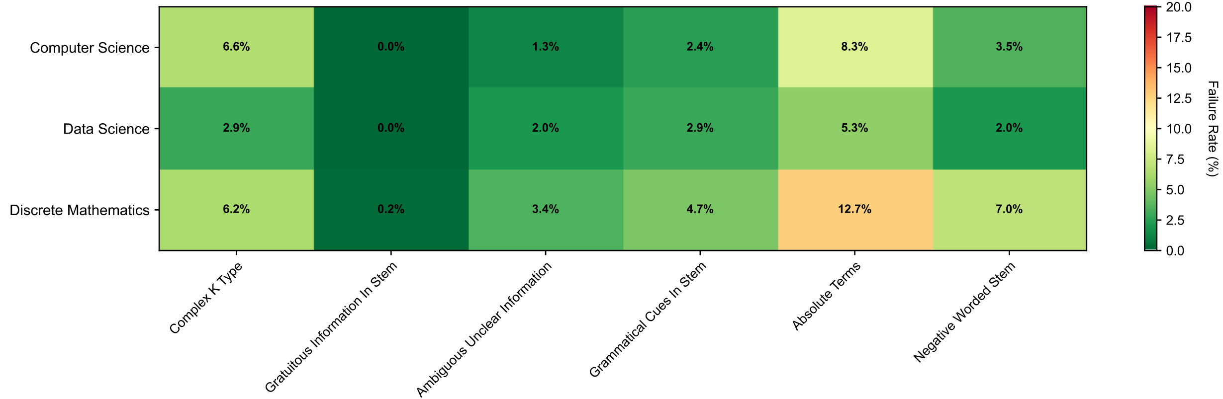
AI Failure Rates on Explicit Prompt Guidelines by Discipline (Green = low failure, Red = high failure)
