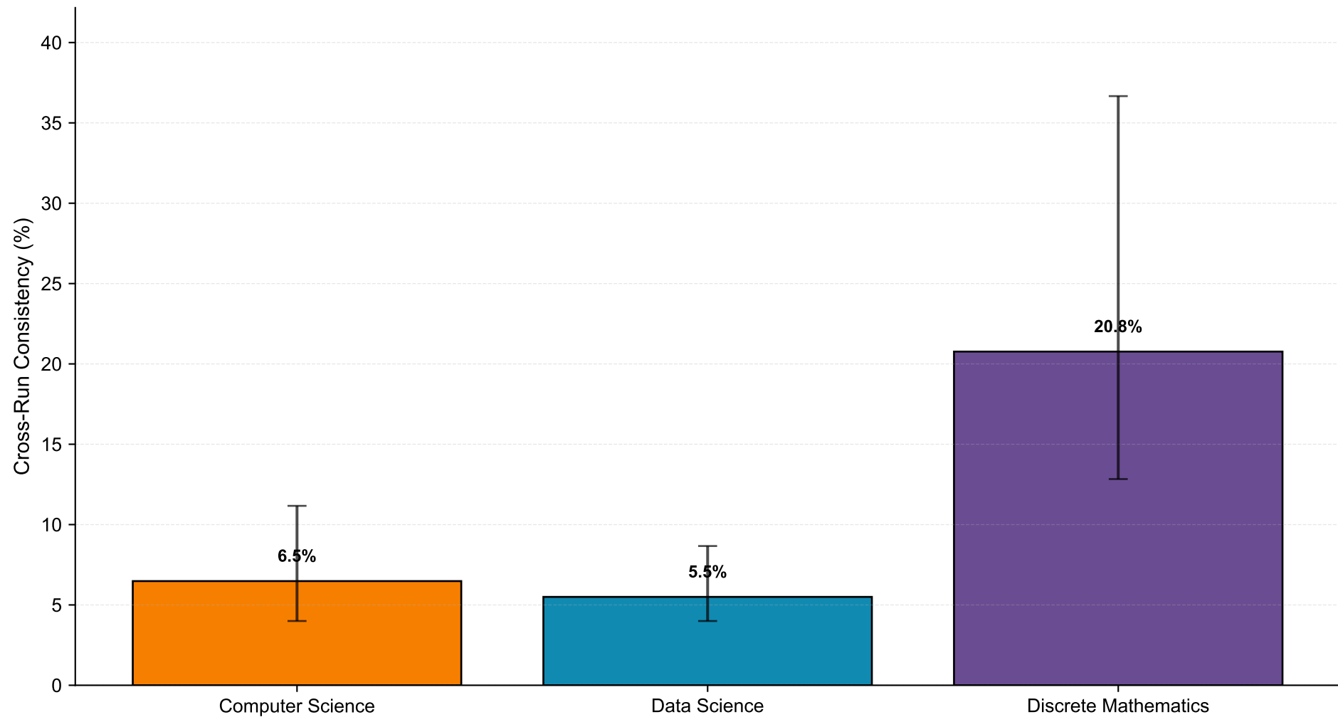
Cross-Run Behavior across multiple runs (Mean with min/max range)
